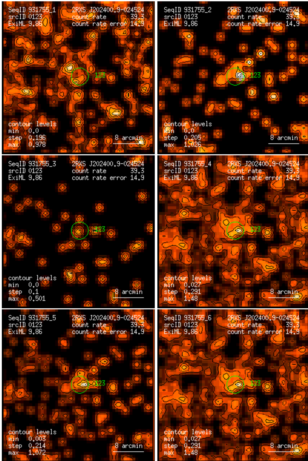
Figure 123: RASS 931755: detection 0123: band rate images, Gaussian filter: (1) PSPC channels 11 – 41, (2) 52 – 90, (3) 91 – 201, (4) 11 – 235, (5) 52 – 201, (6) 11 – 201. Broad band rates in counts/ks. Band rate contour levels in counts/ks/arcmin 2 .
