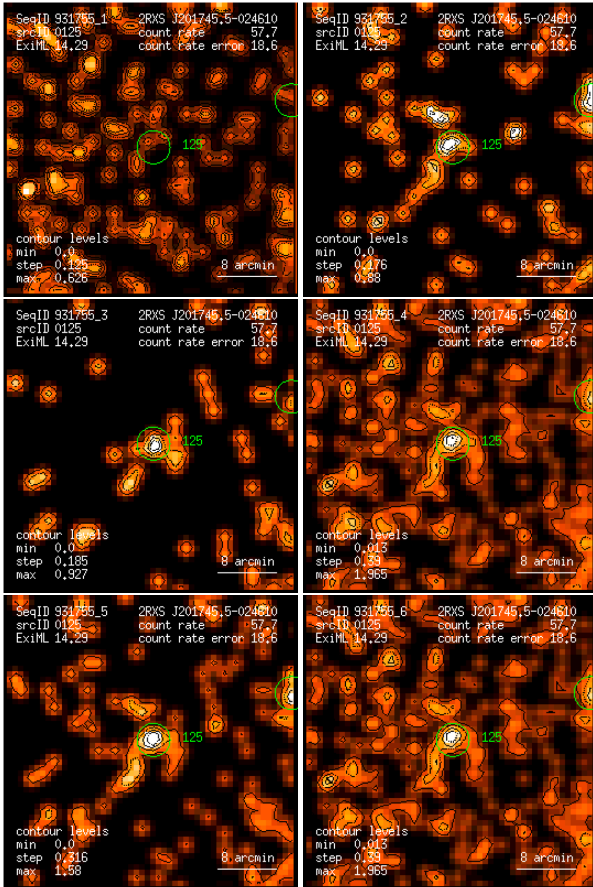
Figure 125: RASS 931755: detection 0125: band rate images, Gaussian filter: (1) PSPC channels 11 – 41, (2) 52 – 90, (3) 91 – 201, (4) 11 – 235, (5) 52 – 201, (6) 11 – 201. Broad band rates in counts/ks. Band rate contour levels in counts/ks/arcmin 2 .
