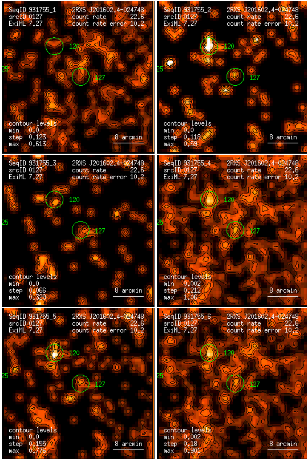
Figure 127: RASS 931755: detection 0127: band rate images, Gaussian filter: (1) PSPC channels 11 – 41, (2) 52 – 90, (3) 91 – 201, (4) 11 – 235, (5) 52 – 201, (6) 11 – 201. Broad band rates in counts/ks. Band rate contour levels in counts/ks/arcmin 2 .
