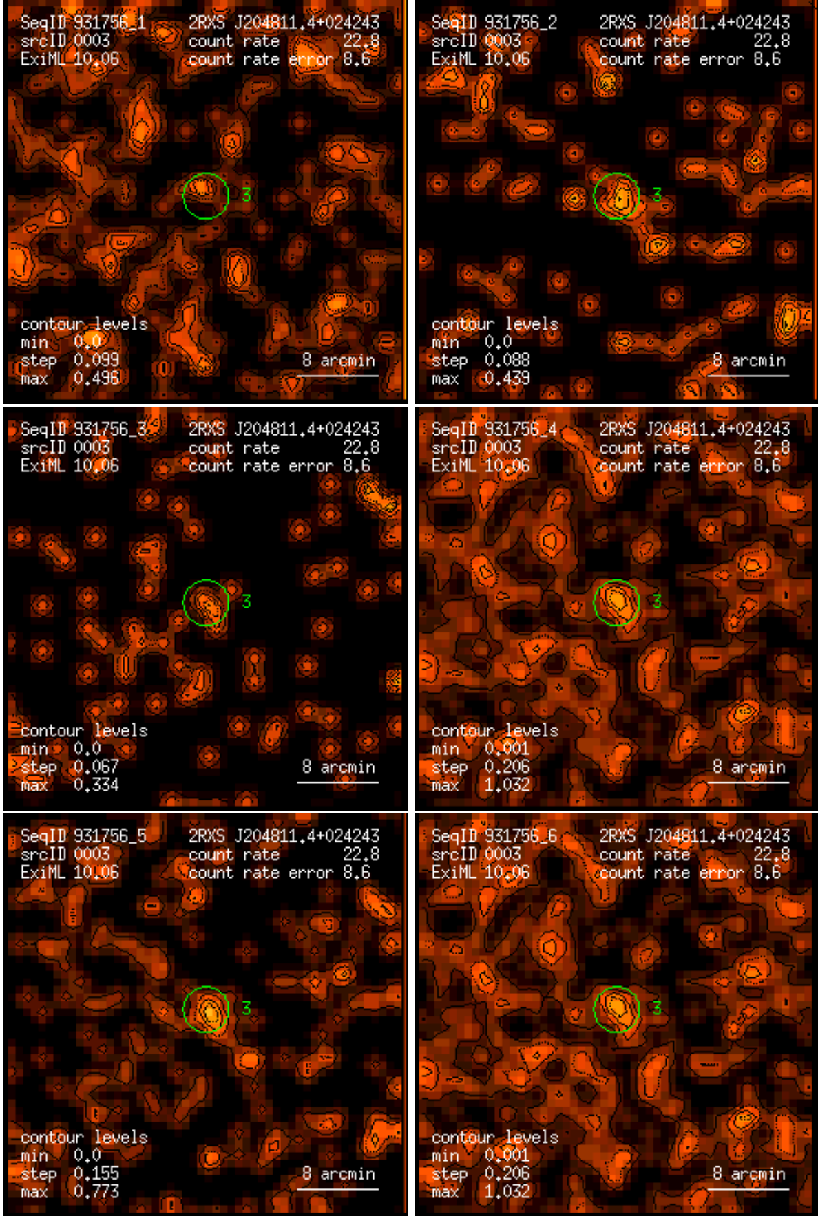
Figure 3: RASS 931756: detection 0003: band rate images, Gaussian filter: (1) PSPC channels 11 – 41, (2) 52 – 90, (3) 91 – 201, (4) 11 – 235, (5) 52 – 201, (6) 11 – 201. Broad band rates in counts/ks. Band rate contour levels in counts/ks/arcmin 2 .
