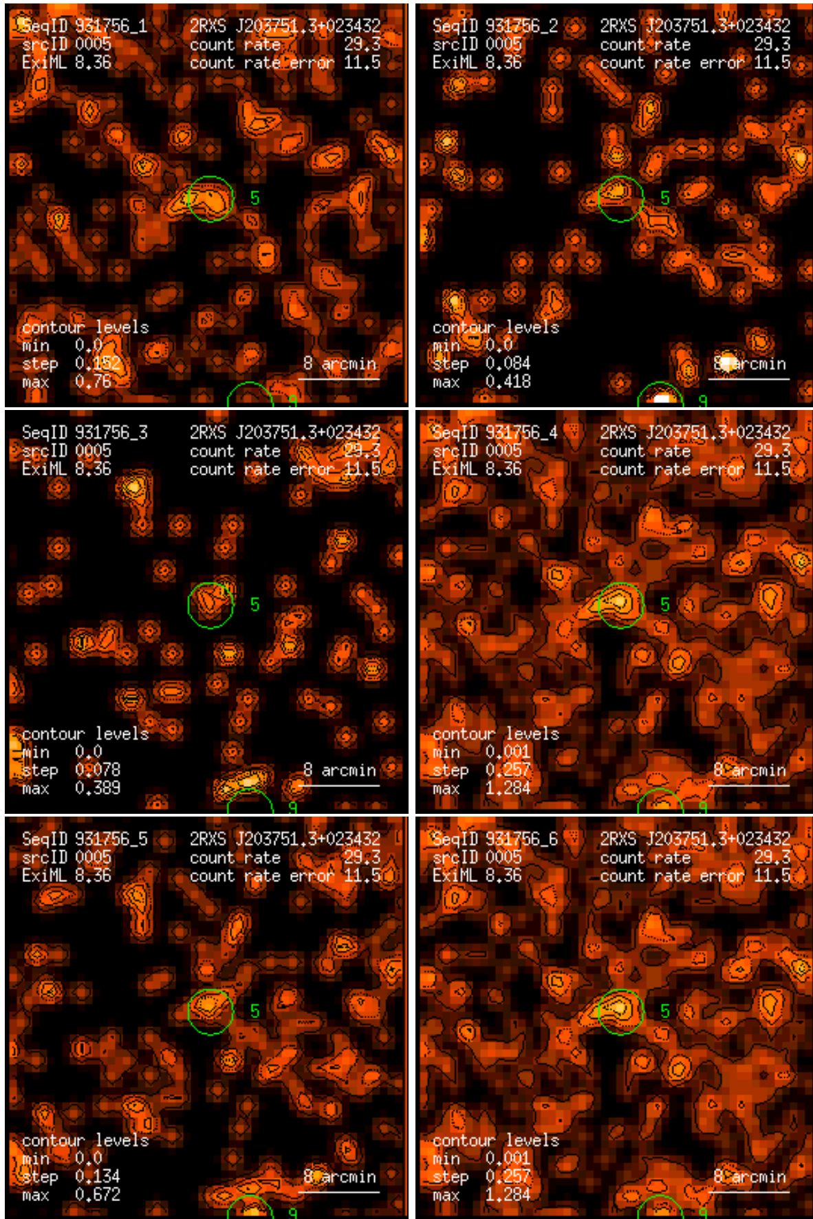
Figure 5: RASS 931756: detection 0005: band rate images, Gaussian filter: (1) PSPC channels 11 – 41, (2) 52 – 90, (3) 91 – 201, (4) 11 – 235, (5) 52 – 201, (6) 11 – 201. Broad band rates in counts/ks. Band rate contour levels in counts/ks/arcmin 2 .
