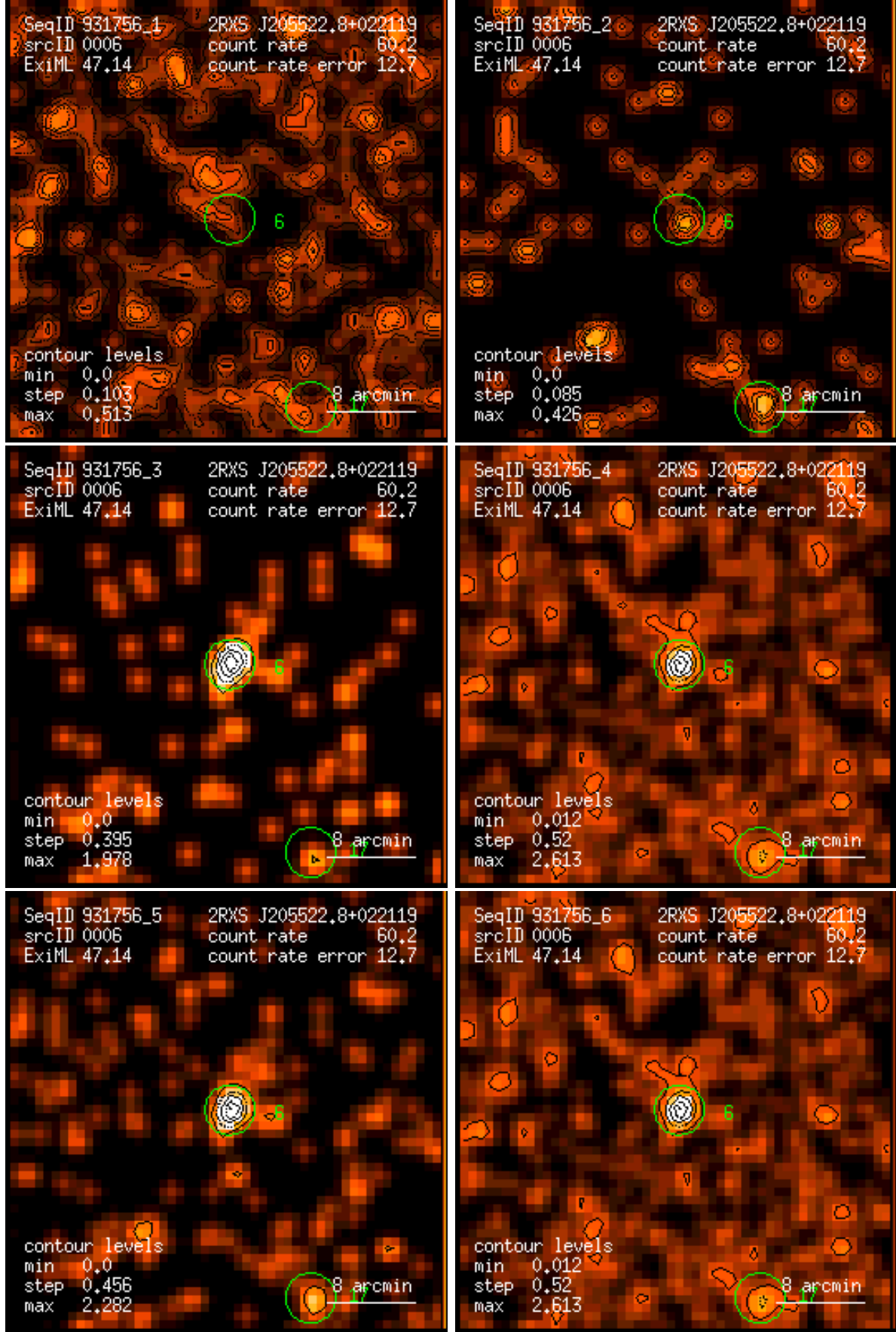
Figure 6: RASS 931756: detection 0006: band rate images, Gaussian filter: (1) PSPC channels 11 – 41, (2) 52 – 90, (3) 91 – 201, (4) 11 – 235, (5) 52 – 201, (6) 11 – 201. Broad band rates in counts/ks. Band rate contour levels in counts/ks/arcmin 2 .
