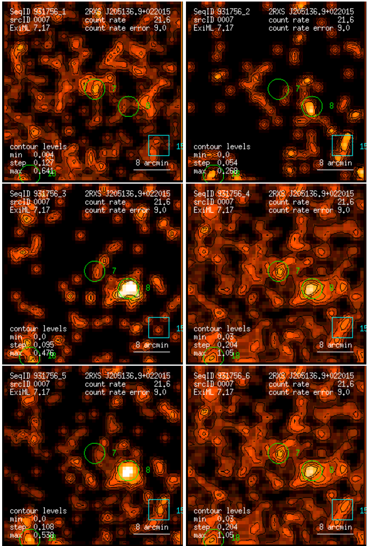
Figure 7: RASS 931756: detection 0007: band rate images, Gaussian filter: (1) PSPC channels 11 – 41, (2) 52 – 90, (3) 91 – 201, (4) 11 – 235, (5) 52 – 201, (6) 11 – 201. Broad band rates in counts/ks. Band rate contour levels in counts/ks/arcmin 2 .
