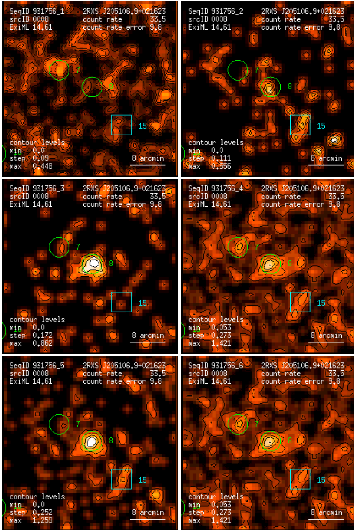
Figure 8: RASS 931756: detection 0008: band rate images, Gaussian filter: (1) PSPC channels 11 – 41, (2) 52 – 90, (3) 91 – 201, (4) 11 – 235, (5) 52 – 201, (6) 11 – 201. Broad band rates in counts/ks. Band rate contour levels in counts/ks/arcmin 2 .
