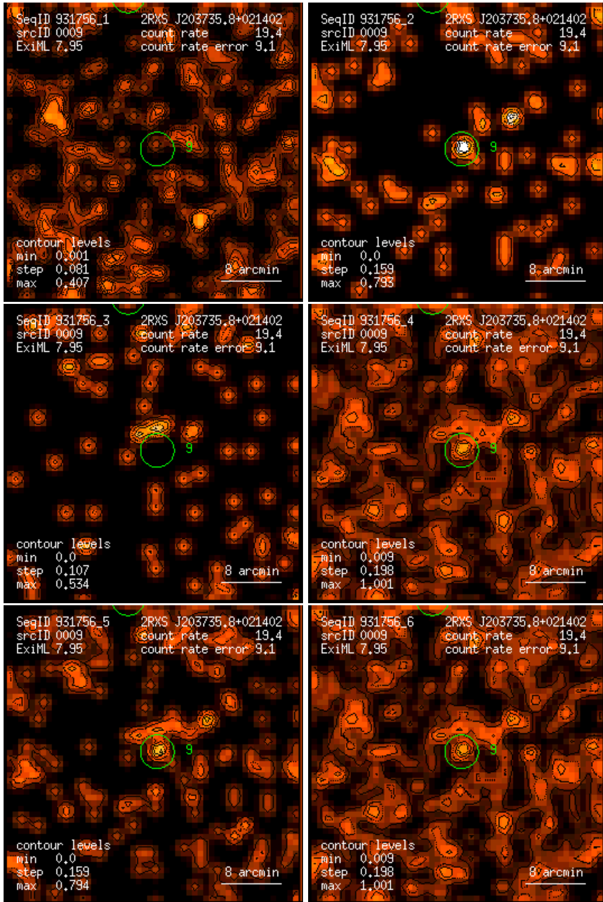
Figure 9: RASS 931756: detection 0009: band rate images, Gaussian filter: (1) PSPC channels 11 – 41, (2) 52 – 90, (3) 91 – 201, (4) 11 – 235, (5) 52 – 201, (6) 11 – 201. Broad band rates in counts/ks. Band rate contour levels in counts/ks/arcmin 2 .
