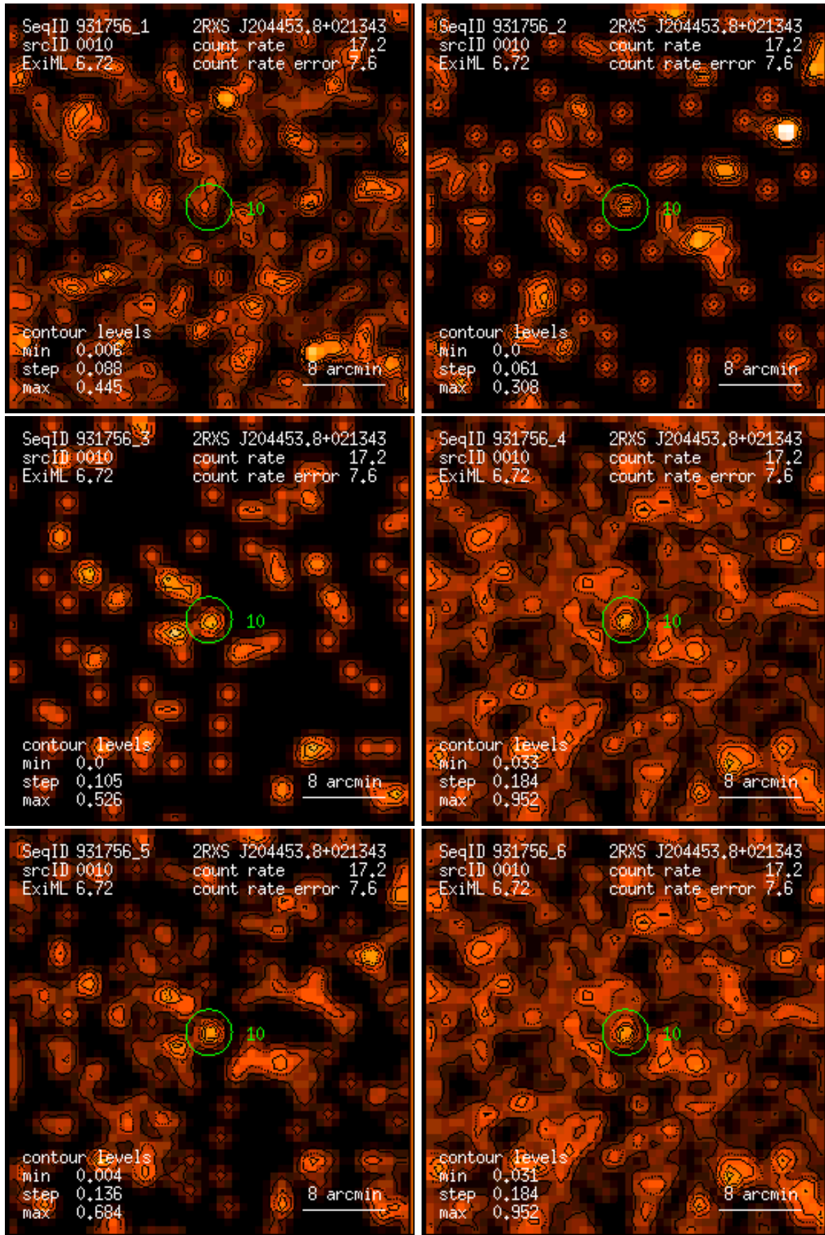
Figure 10: RASS 931756: detection 0010: band rate images, Gaussian filter: (1) PSPC channels 11 – 41, (2) 52 – 90, (3) 91 – 201, (4) 11 – 235, (5) 52 – 201, (6) 11 – 201. Broad band rates in counts/ks. Band rate contour levels in counts/ks/arcmin 2 .
