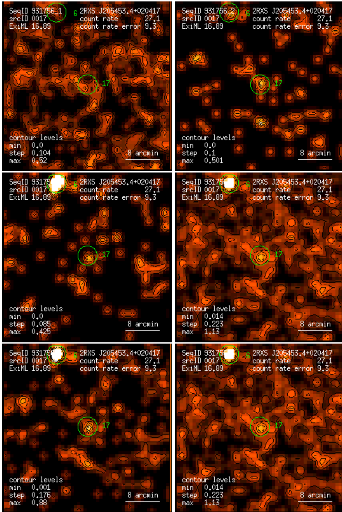
Figure 17: RASS 931756: detection 0017: band rate images, Gaussian filter: (1) PSPC channels 11 – 41, (2) 52 – 90, (3) 91 – 201, (4) 11 – 235, (5) 52 – 201, (6) 11 – 201. Broad band rates in counts/ks. Band rate contour levels in counts/ks/arcmin 2 .
