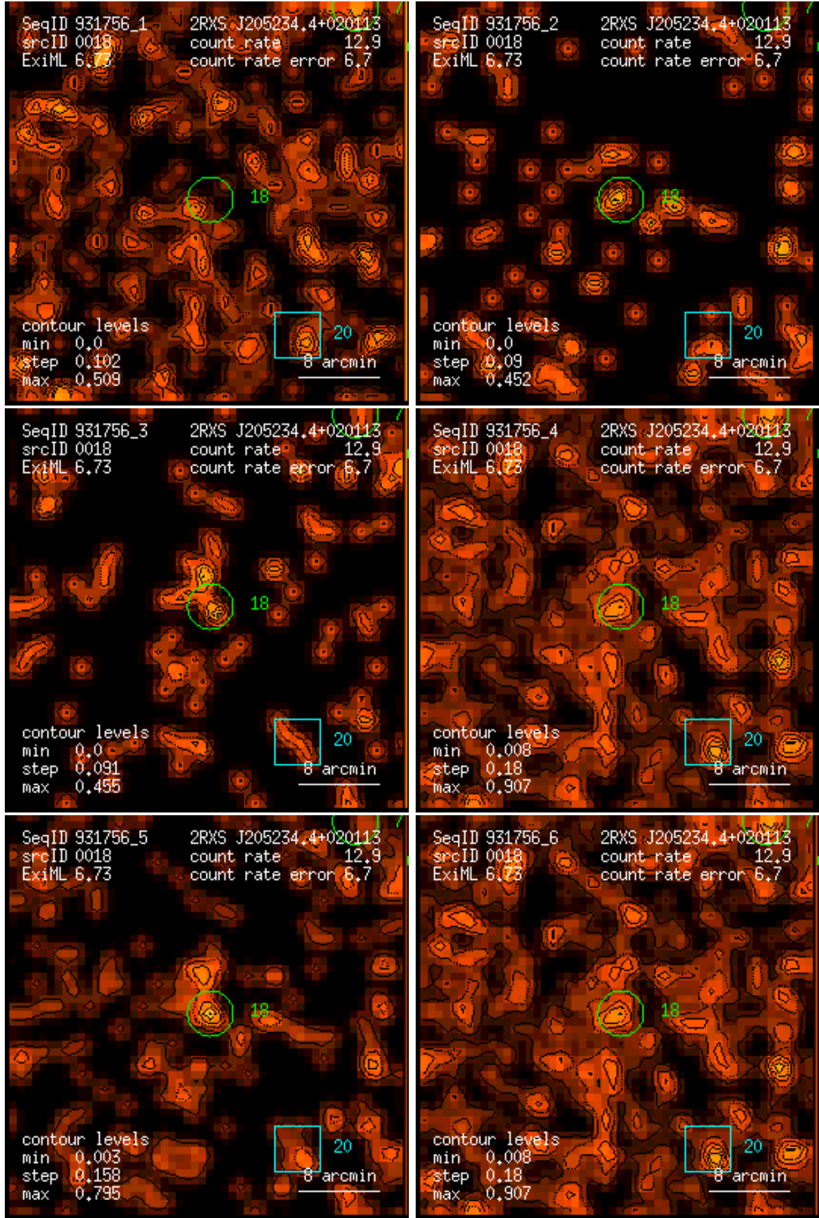
Figure 18: RASS 931756: detection 0018: band rate images, Gaussian filter: (1) PSPC channels 11 – 41, (2) 52 – 90, (3) 91 – 201, (4) 11 – 235, (5) 52 – 201, (6) 11 – 201. Broad band rates in counts/ks. Band rate contour levels in counts/ks/arcmin 2 .
