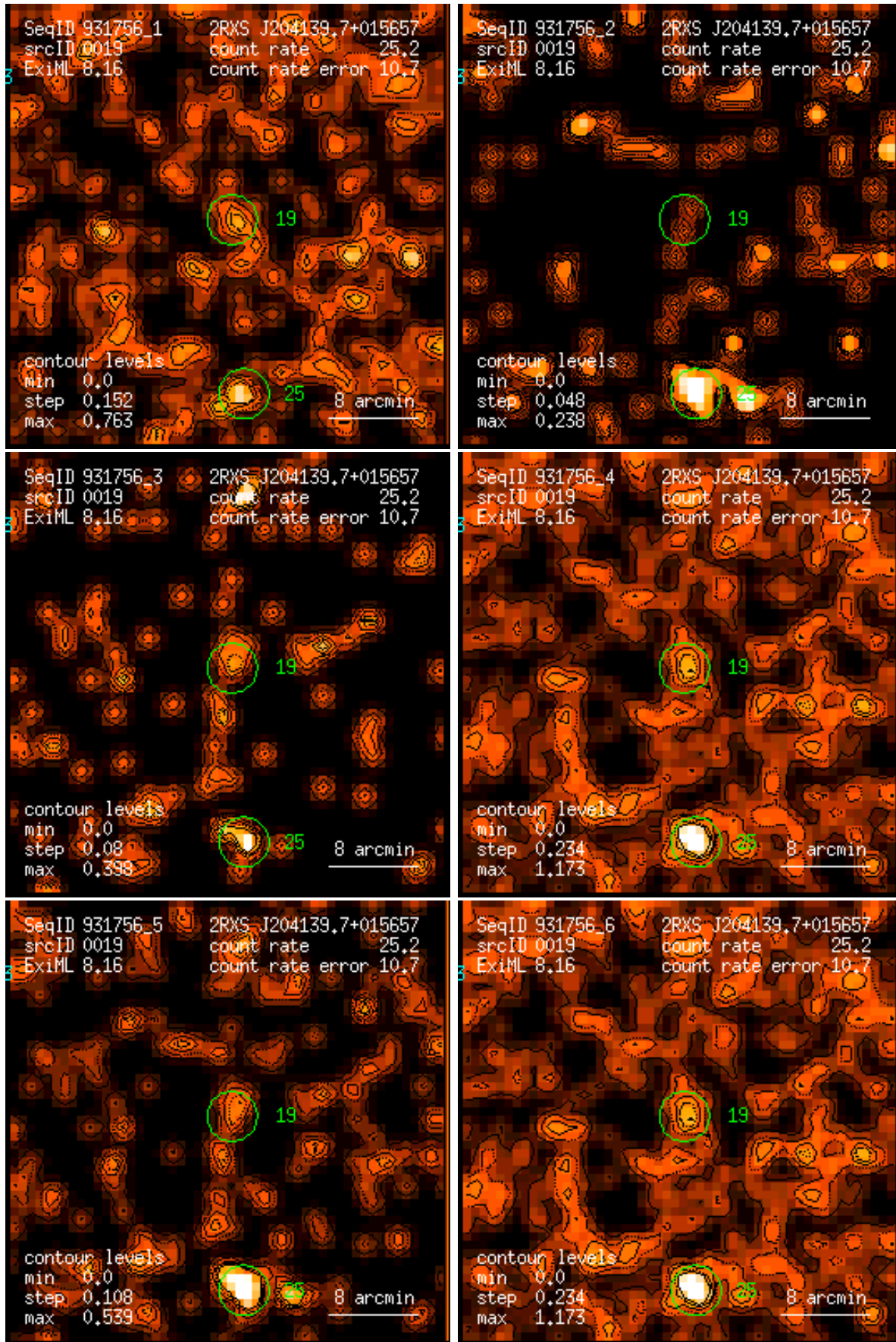
Figure 19: RASS 931756: detection 0019: band rate images, Gaussian filter: (1) PSPC channels 11 – 41, (2) 52 – 90, (3) 91 – 201, (4) 11 – 235, (5) 52 – 201, (6) 11 – 201. Broad band rates in counts/ks. Band rate contour levels in counts/ks/arcmin 2 .
