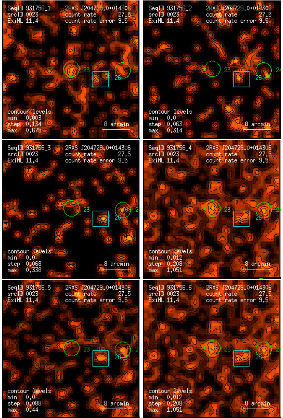
Figure 23: RASS 931756: detection 0023: band rate images, Gaussian filter: (1) PSPC channels 11 – 41, (2) 52 – 90, (3) 91 – 201, (4) 11 – 235, (5) 52 – 201, (6) 11 – 201. Broad band rates in counts/ks. Band rate contour levels in counts/ks/arcmin 2 .
