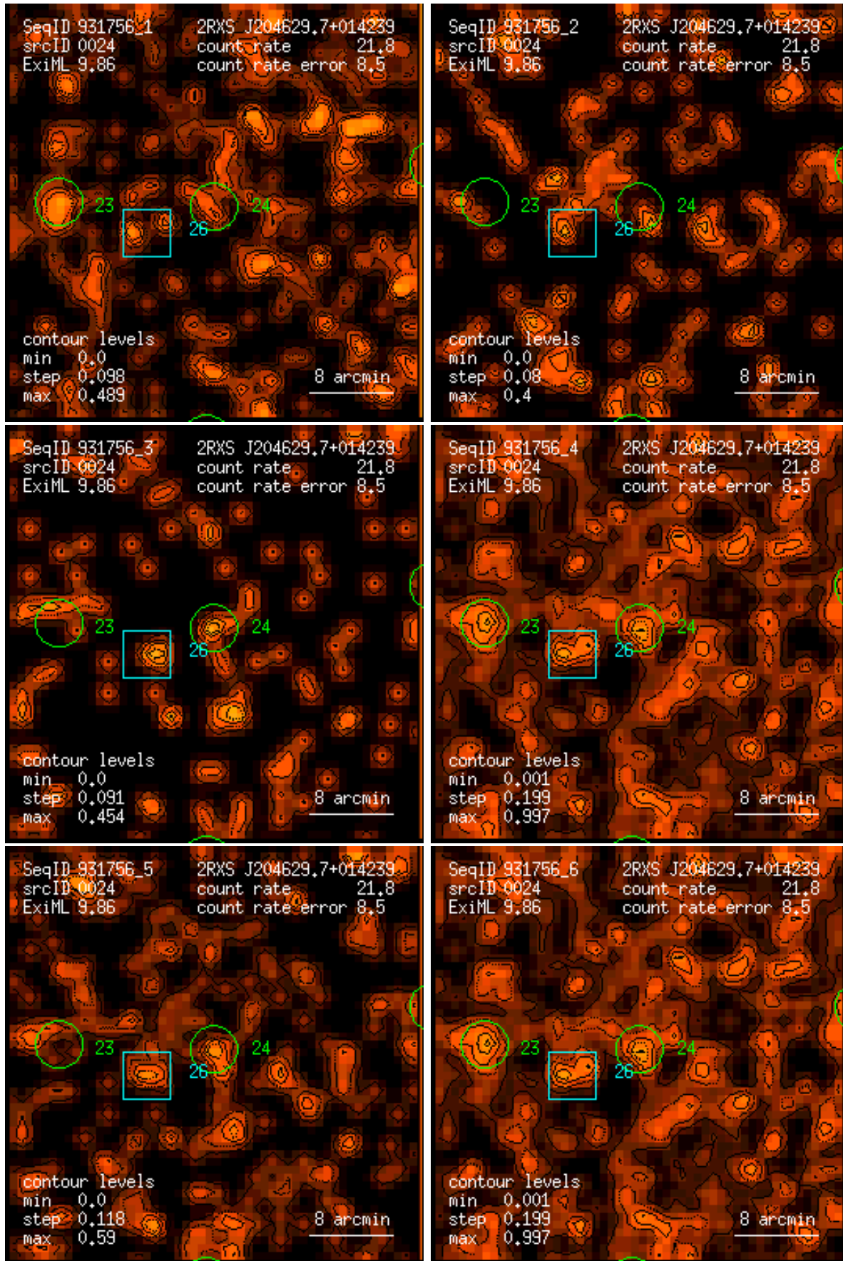
Figure 24: RASS 931756: detection 0024: band rate images, Gaussian filter: (1) PSPC channels 11 – 41, (2) 52 – 90, (3) 91 – 201, (4) 11 – 235, (5) 52 – 201, (6) 11 – 201. Broad band rates in counts/ks. Band rate contour levels in counts/ks/arcmin 2 .
