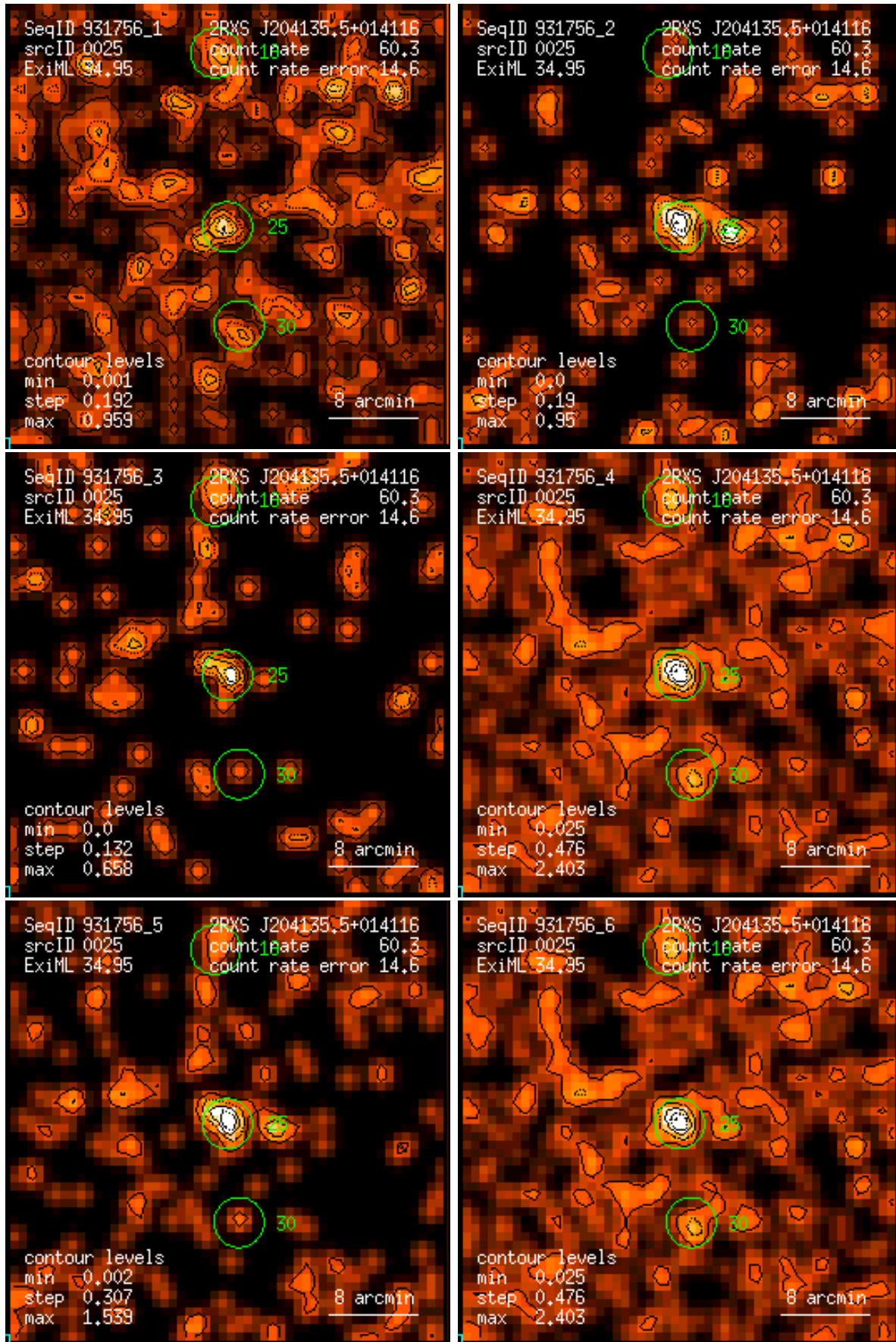
Figure 25: RASS 931756: detection 0025: band rate images, Gaussian filter: (1) PSPC channels 11 – 41, (2) 52 – 90, (3) 91 – 201, (4) 11 – 235, (5) 52 – 201, (6) 11 – 201. Broad band rates in counts/ks. Band rate contour levels in counts/ks/arcmin 2 .
