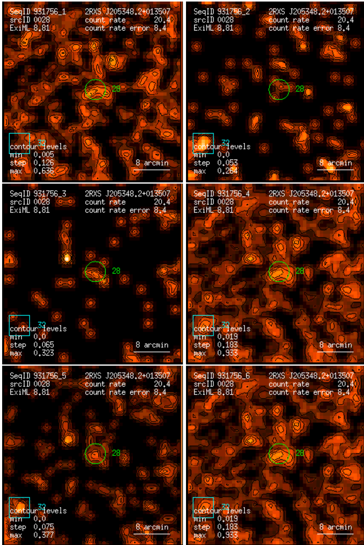
Figure 28: RASS 931756: detection 0028: band rate images, Gaussian filter: (1) PSPC channels 11 – 41, (2) 52 – 90, (3) 91 – 201, (4) 11 – 235, (5) 52 – 201, (6) 11 – 201. Broad band rates in counts/ks. Band rate contour levels in counts/ks/arcmin 2 .
