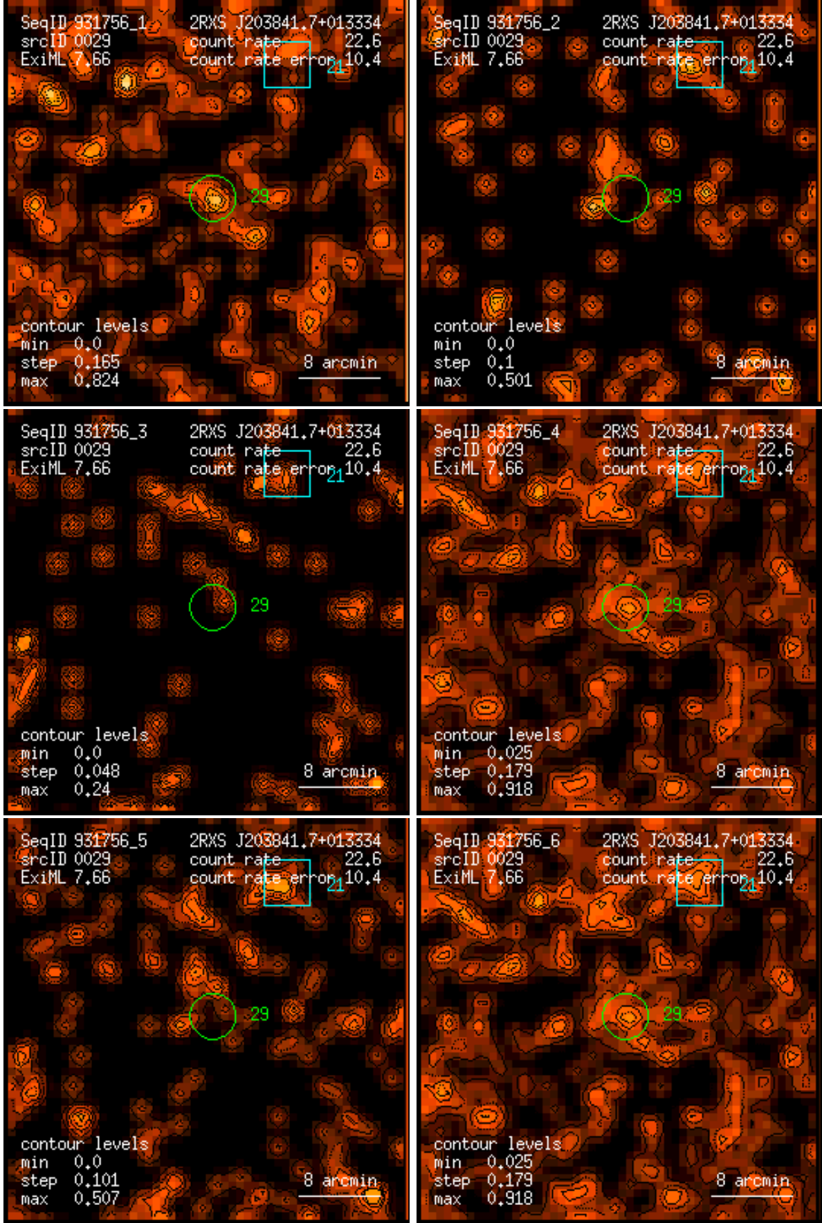
Figure 29: RASS 931756: detection 0029: band rate images, Gaussian filter: (1) PSPC channels 11 – 41, (2) 52 – 90, (3) 91 – 201, (4) 11 – 235, (5) 52 – 201, (6) 11 – 201. Broad band rates in counts/ks. Band rate contour levels in counts/ks/arcmin 2 .
