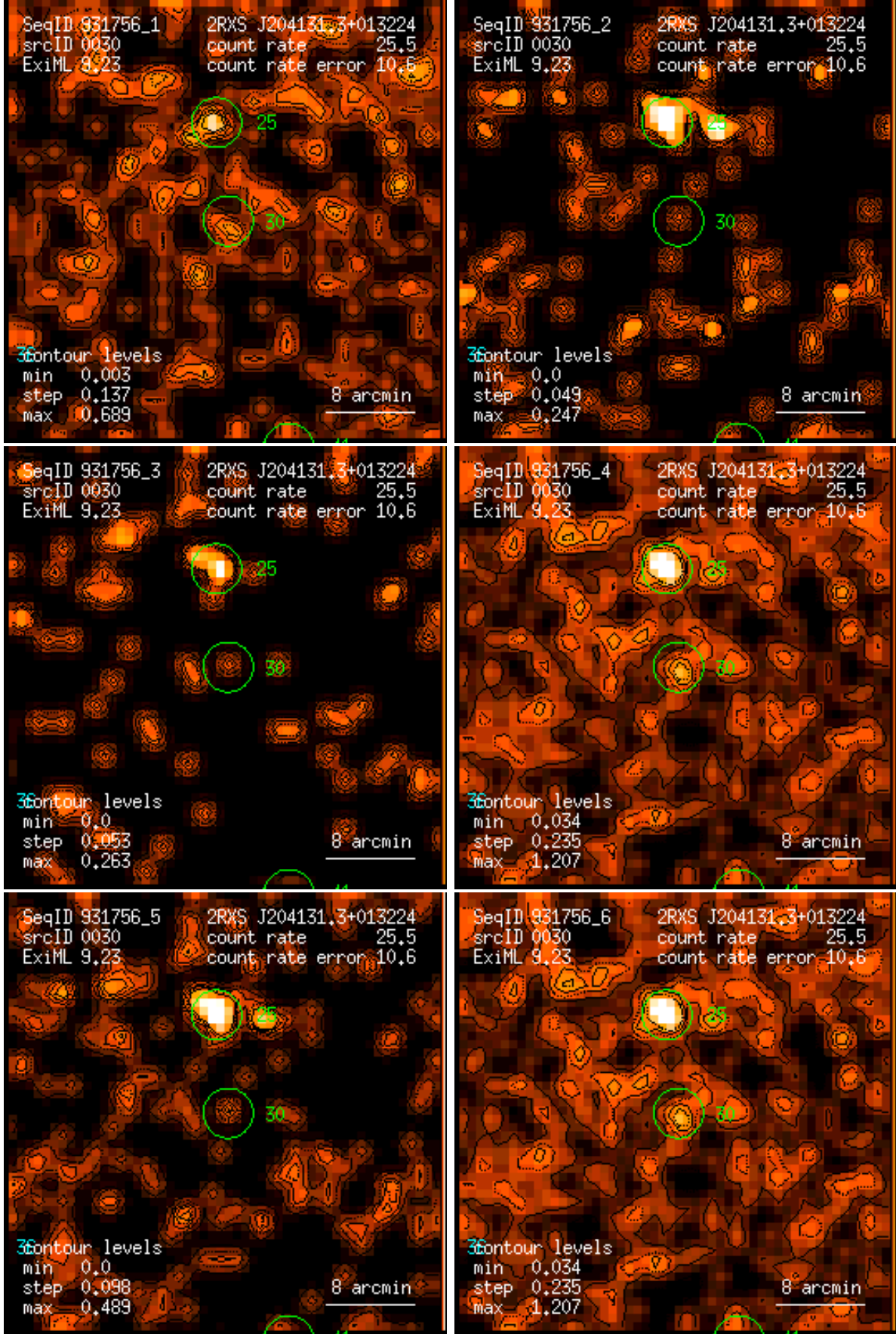
Figure 30: RASS 931756: detection 0030: band rate images, Gaussian filter: (1) PSPC channels 11 – 41, (2) 52 – 90, (3) 91 – 201, (4) 11 – 235, (5) 52 – 201, (6) 11 – 201. Broad band rates in counts/ks. Band rate contour levels in counts/ks/arcmin 2 .
