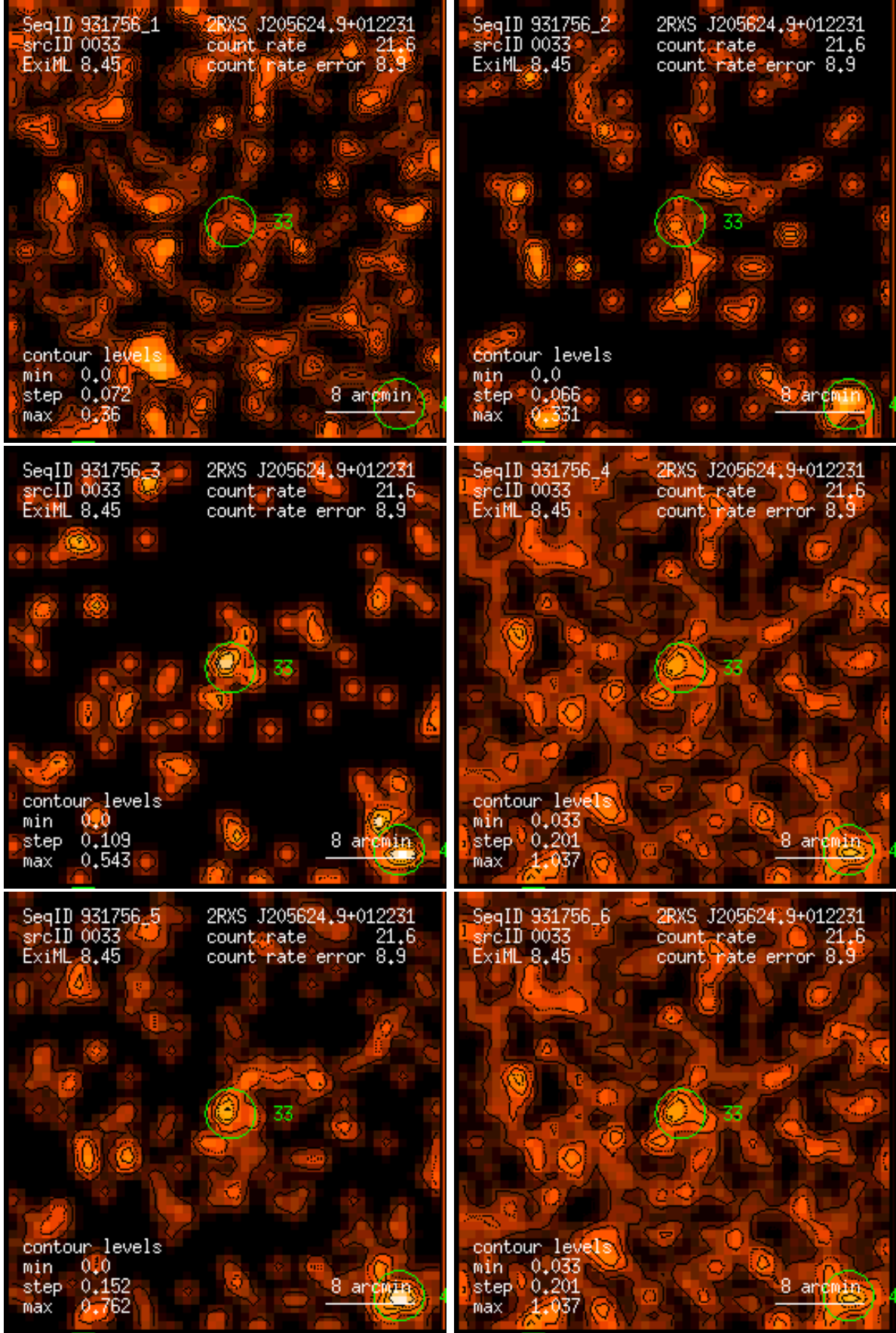
Figure 33: RASS 931756: detection 0033: band rate images, Gaussian filter: (1) PSPC channels 11 – 41, (2) 52 – 90, (3) 91 – 201, (4) 11 – 235, (5) 52 – 201, (6) 11 – 201. Broad band rates in counts/ks. Band rate contour levels in counts/ks/arcmin 2 .
