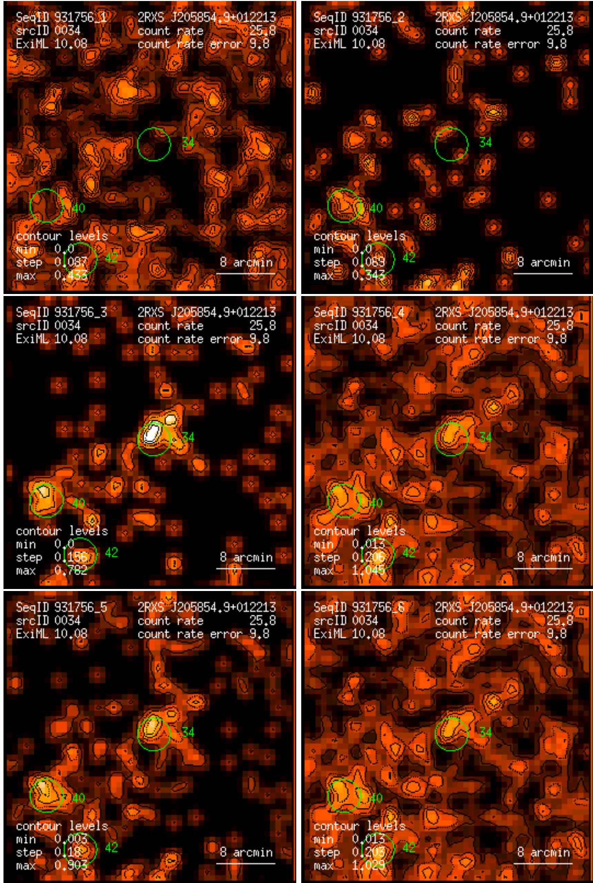
Figure 34: RASS 931756: detection 0034: band rate images, Gaussian filter: (1) PSPC channels 11 – 41, (2) 52 – 90, (3) 91 – 201, (4) 11 – 235, (5) 52 – 201, (6) 11 – 201. Broad band rates in counts/ks. Band rate contour levels in counts/ks/arcmin 2 .
