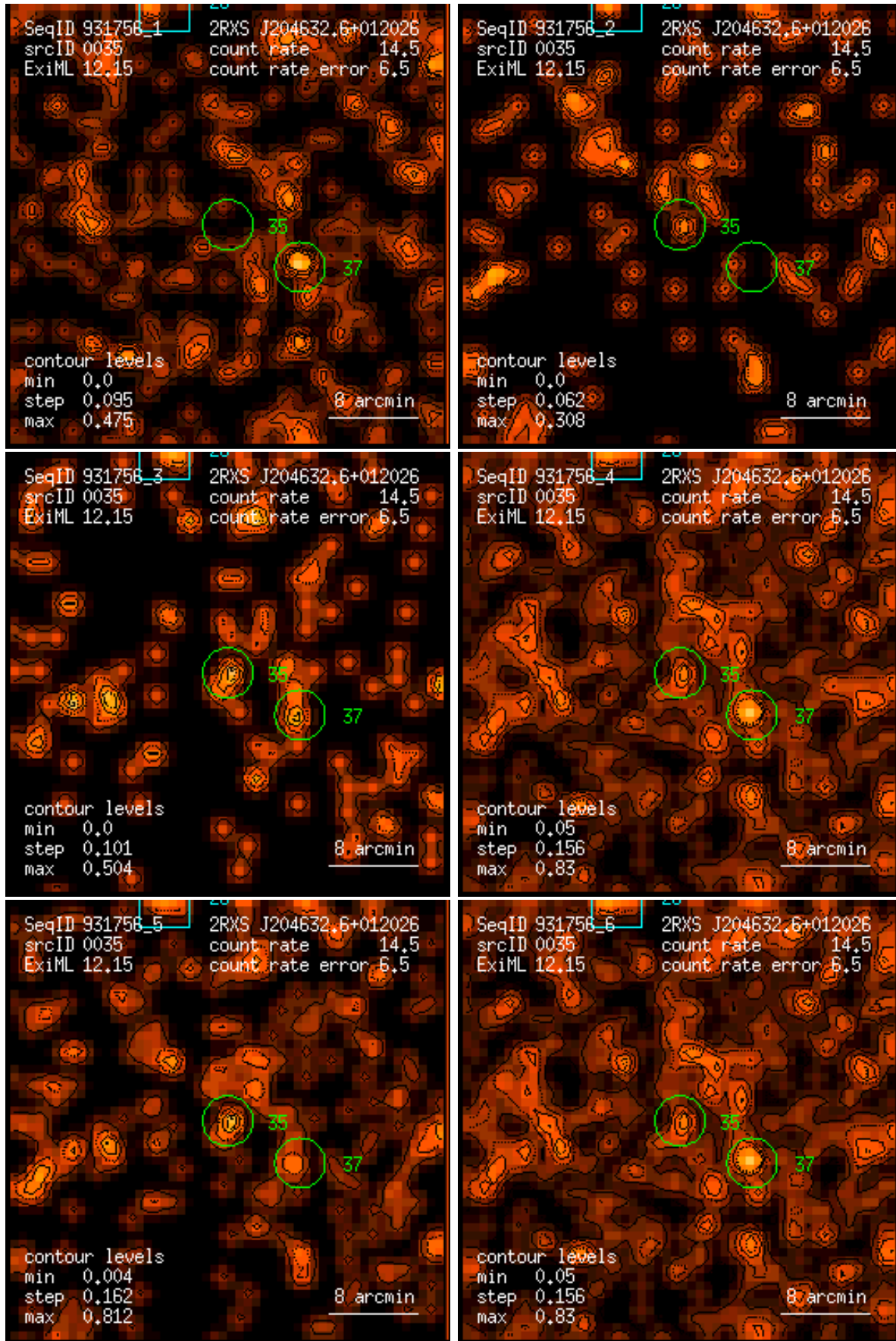
Figure 35: RASS 931756: detection 0035: band rate images, Gaussian filter: (1) PSPC channels 11 – 41, (2) 52 – 90, (3) 91 – 201, (4) 11 – 235, (5) 52 – 201, (6) 11 – 201. Broad band rates in counts/ks. Band rate contour levels in counts/ks/arcmin 2 .
