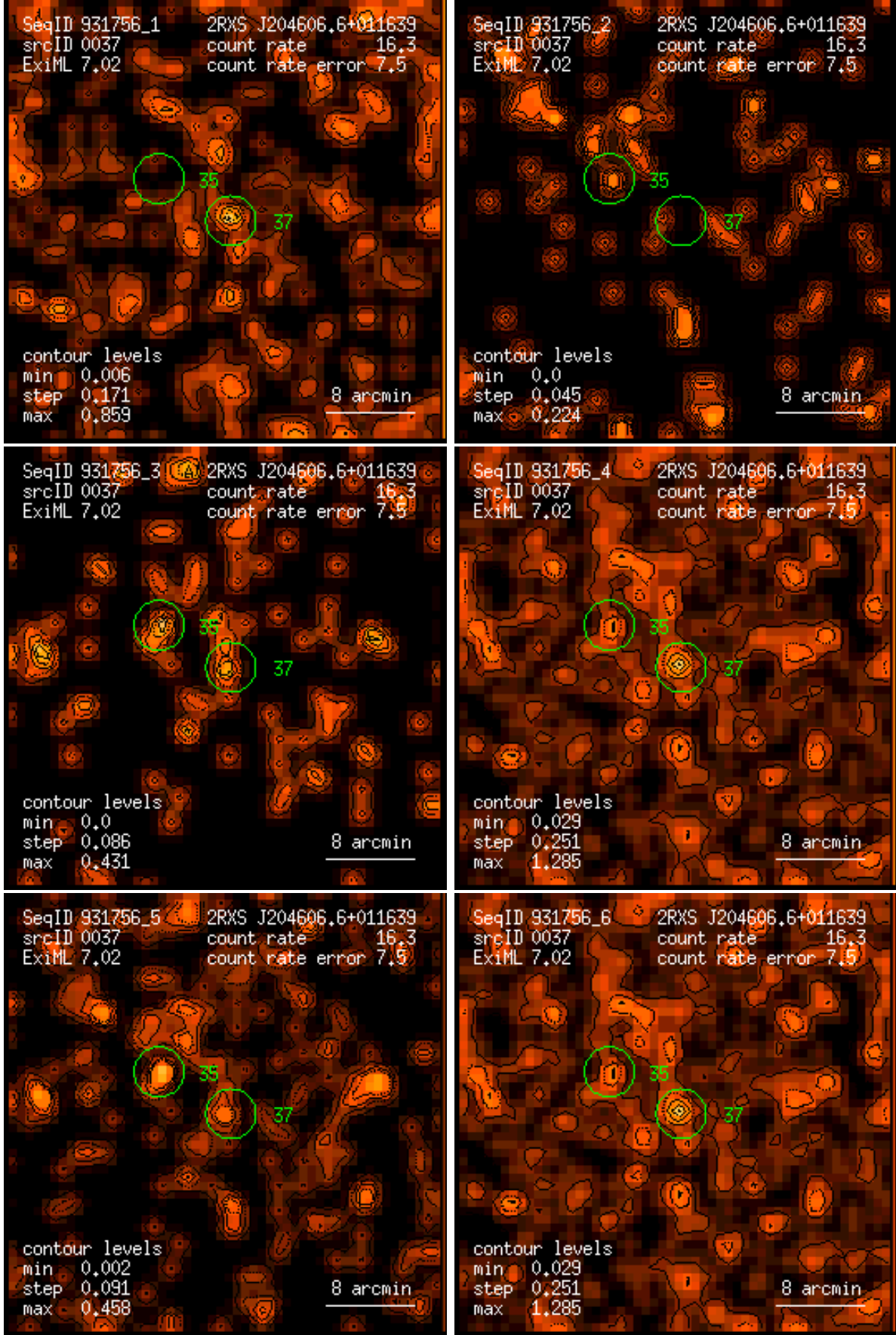
Figure 37: RASS 931756: detection 0037: band rate images, Gaussian filter: (1) PSPC channels 11 – 41, (2) 52 – 90, (3) 91 – 201, (4) 11 – 235, (5) 52 – 201, (6) 11 – 201. Broad band rates in counts/ks. Band rate contour levels in counts/ks/arcmin 2 .
