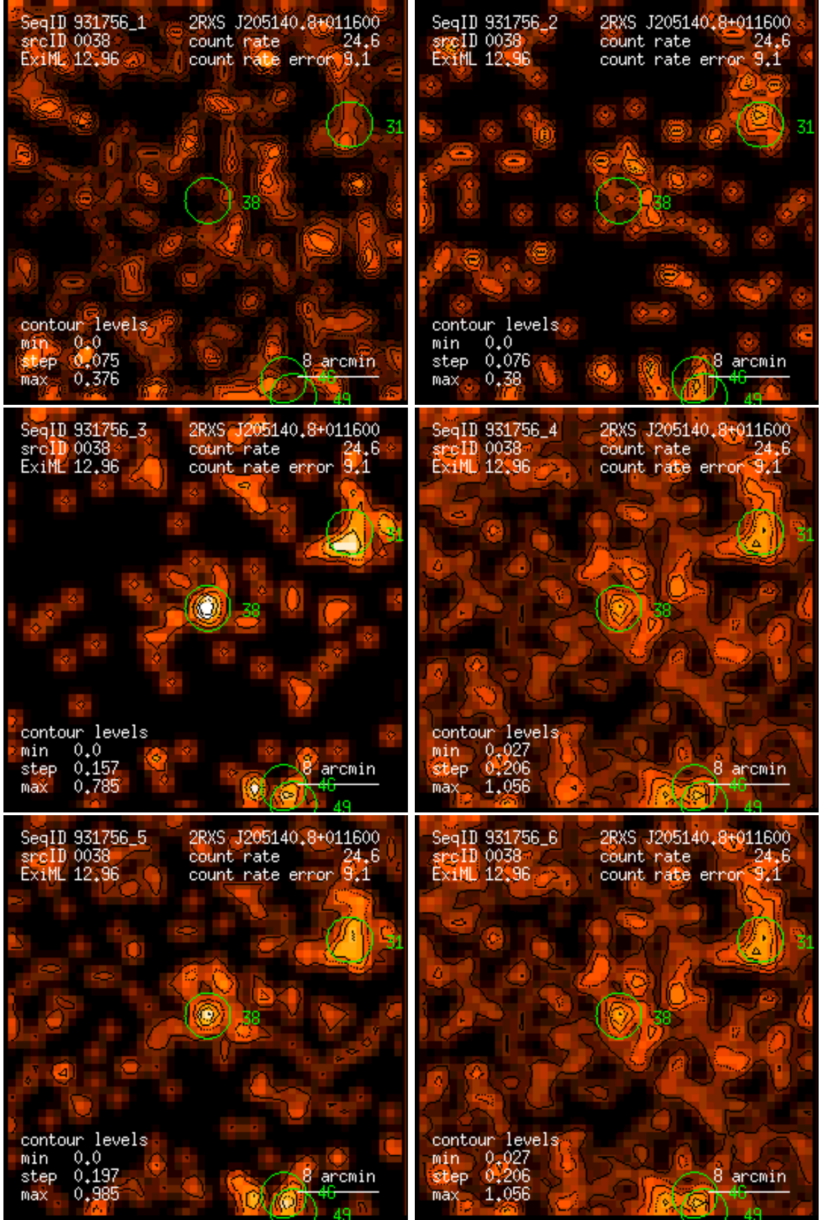
Figure 38: RASS 931756: detection 0038: band rate images, Gaussian filter: (1) PSPC channels 11 – 41, (2) 52 – 90, (3) 91 – 201, (4) 11 – 235, (5) 52 – 201, (6) 11 – 201. Broad band rates in counts/ks. Band rate contour levels in counts/ks/arcmin 2 .
