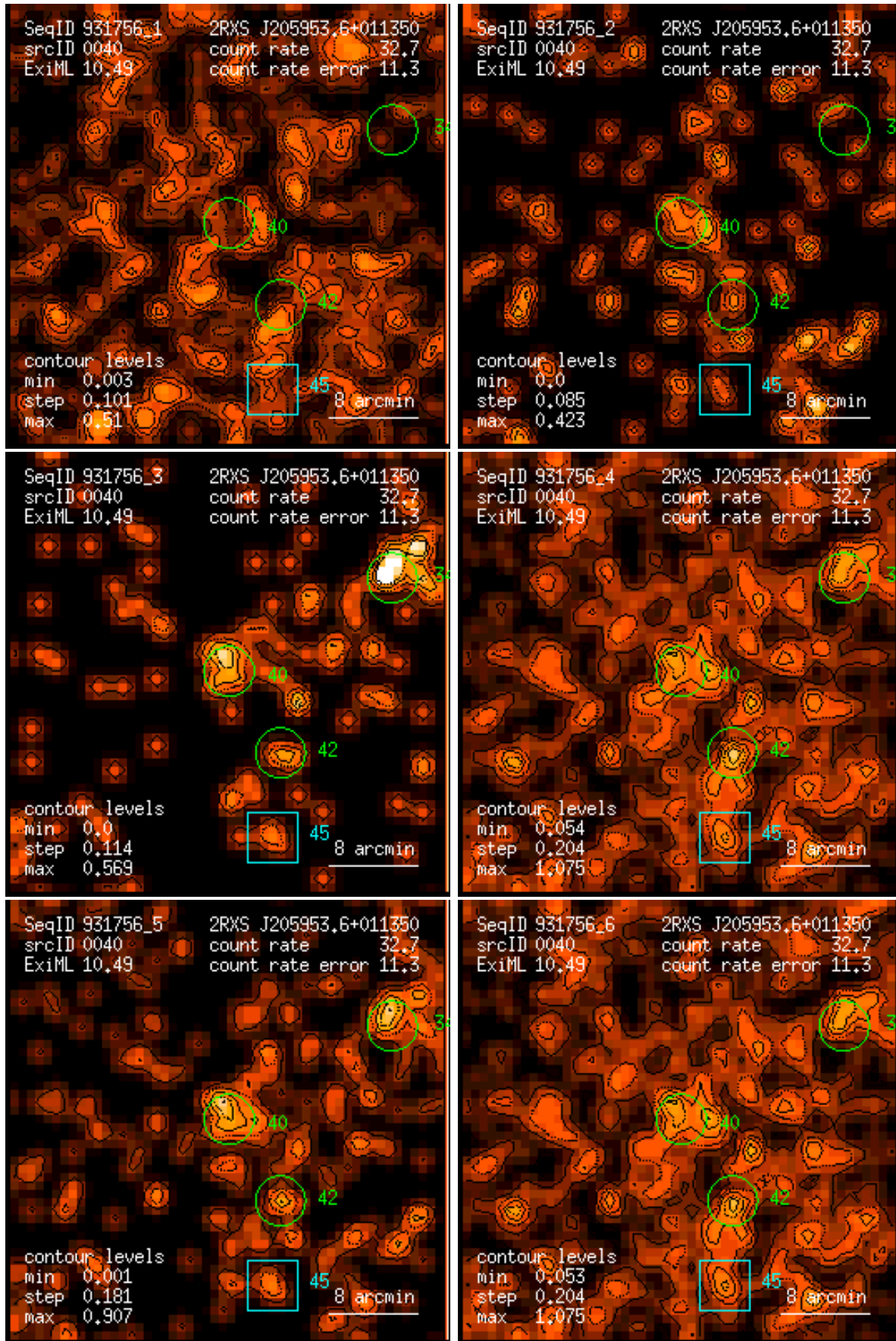
Figure 40: RASS 931756: detection 0040: band rate images, Gaussian filter: (1) PSPC channels 11 – 41, (2) 52 – 90, (3) 91 – 201, (4) 11 – 235, (5) 52 – 201, (6) 11 – 201. Broad band rates in counts/ks. Band rate contour levels in counts/ks/arcmin 2 .
