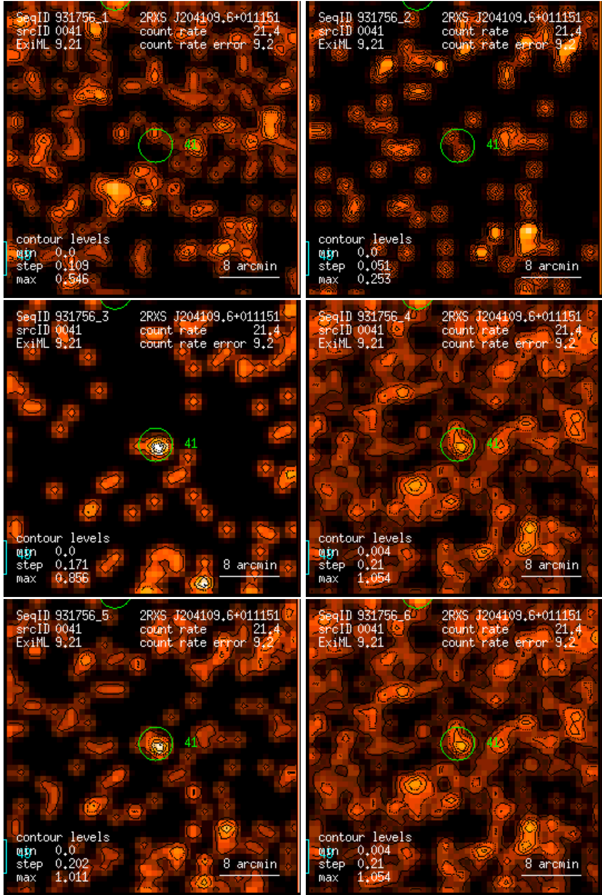
Figure 41: RASS 931756: detection 0041: band rate images, Gaussian filter: (1) PSPC channels 11 – 41, (2) 52 – 90, (3) 91 – 201, (4) 11 – 235, (5) 52 – 201, (6) 11 – 201. Broad band rates in counts/ks. Band rate contour levels in counts/ks/arcmin 2 .
