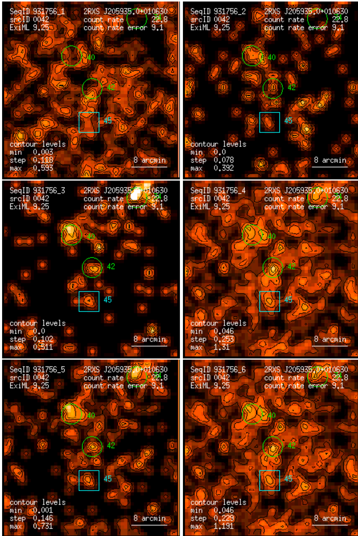
Figure 42: RASS 931756: detection 0042: band rate images, Gaussian filter: (1) PSPC channels 11 – 41, (2) 52 – 90, (3) 91 – 201, (4) 11 – 235, (5) 52 – 201, (6) 11 – 201. Broad band rates in counts/ks. Band rate contour levels in counts/ks/arcmin 2 .
