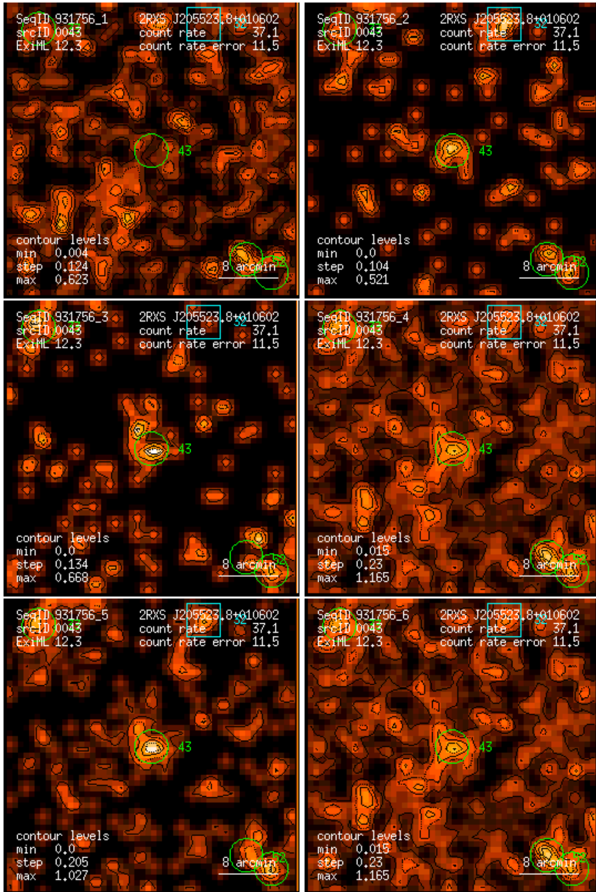
Figure 43: RASS 931756: detection 0043: band rate images, Gaussian filter: (1) PSPC channels 11 – 41, (2) 52 – 90, (3) 91 – 201, (4) 11 – 235, (5) 52 – 201, (6) 11 – 201. Broad band rates in counts/ks. Band rate contour levels in counts/ks/arcmin 2 .
