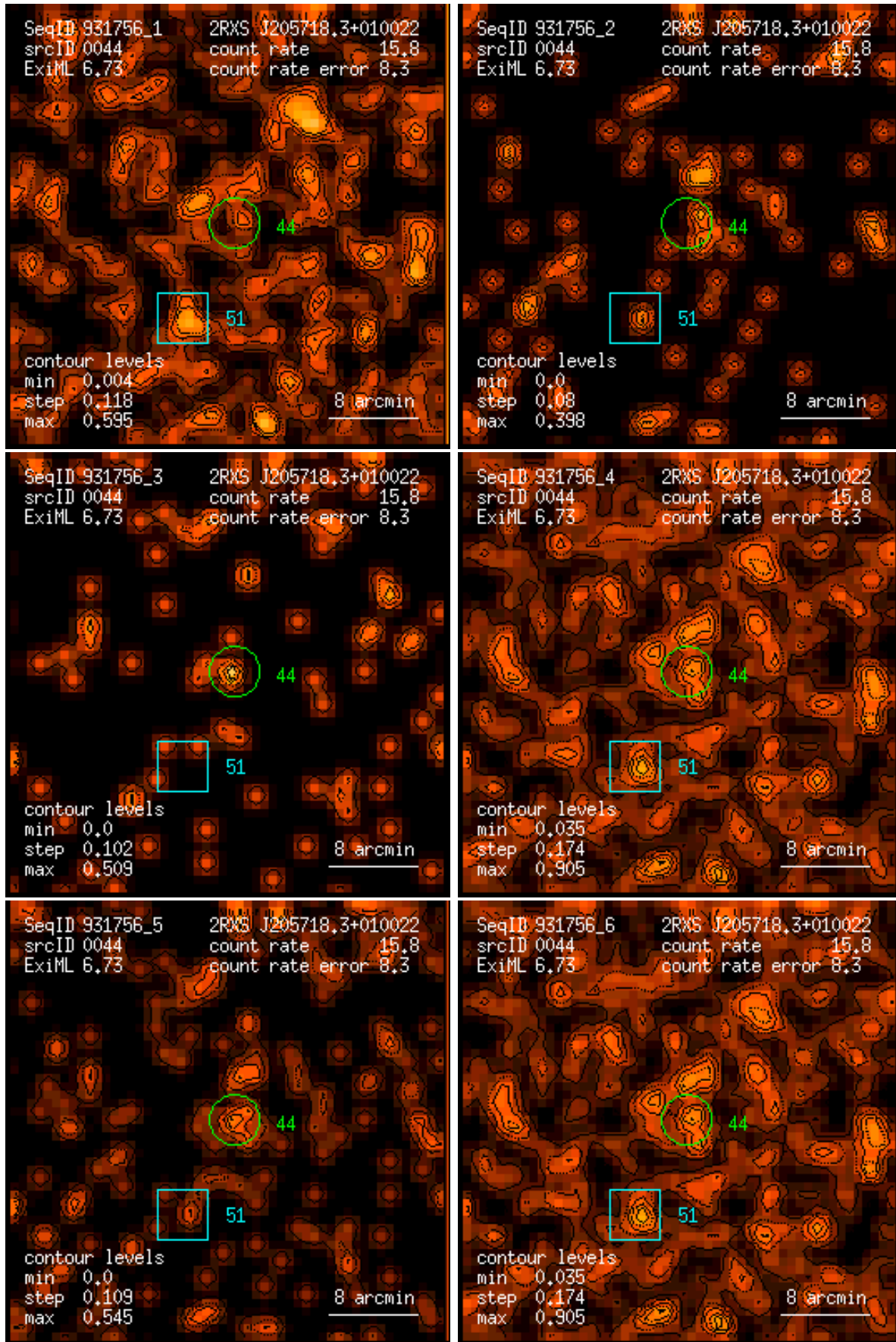
Figure 44: RASS 931756: detection 0044: band rate images, Gaussian filter: (1) PSPC channels 11 – 41, (2) 52 – 90, (3) 91 – 201, (4) 11 – 235, (5) 52 – 201, (6) 11 – 201. Broad band rates in counts/ks. Band rate contour levels in counts/ks/arcmin 2 .
