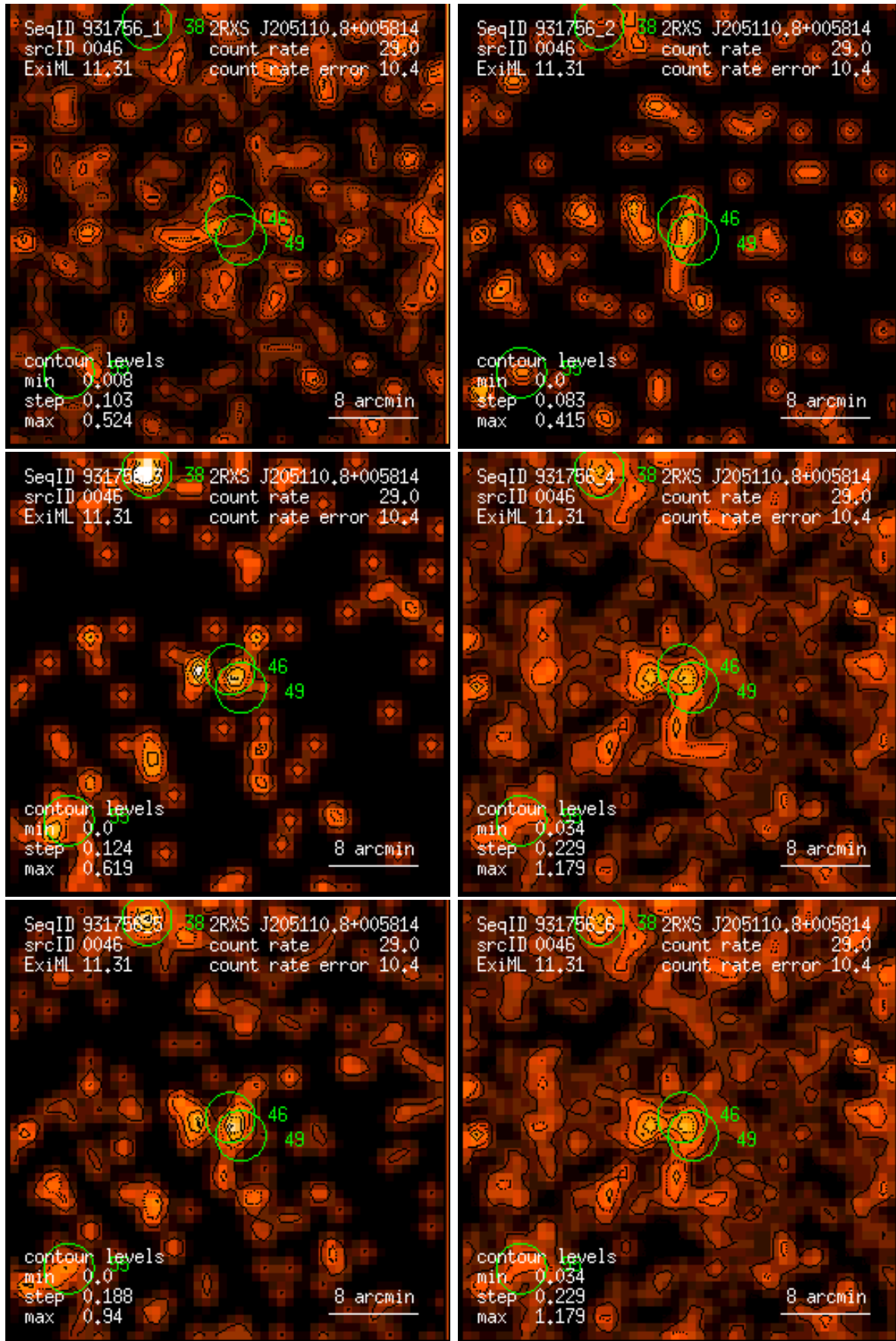
Figure 46: RASS 931756: detection 0046: band rate images, Gaussian filter: (1) PSPC channels 11 – 41, (2) 52 – 90, (3) 91 – 201, (4) 11 – 235, (5) 52 – 201, (6) 11 – 201. Broad band rates in counts/ks. Band rate contour levels in counts/ks/arcmin 2 .
