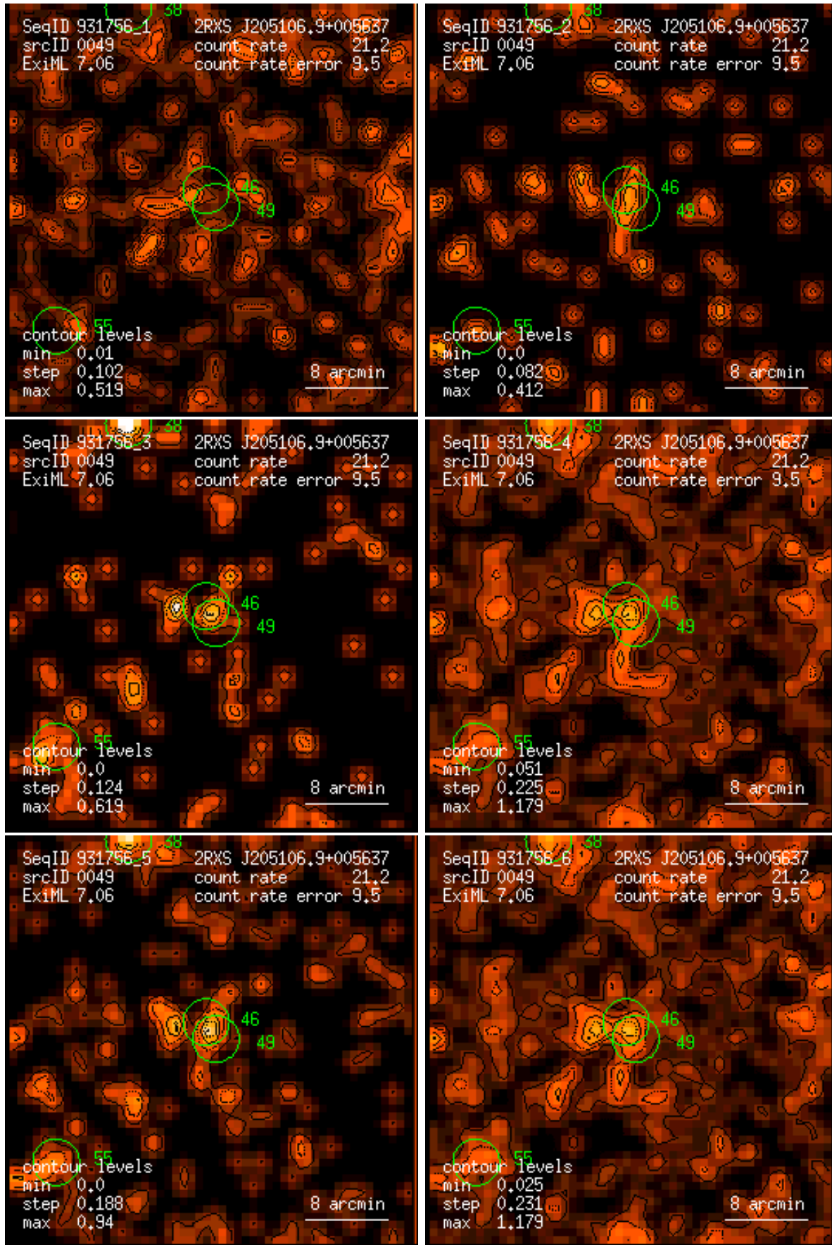
Figure 49: RASS 931756: detection 0049: band rate images, Gaussian filter: (1) PSPC channels 11 – 41, (2) 52 – 90, (3) 91 – 201, (4) 11 – 235, (5) 52 – 201, (6) 11 – 201. Broad band rates in counts/ks. Band rate contour levels in counts/ks/arcmin 2 .
