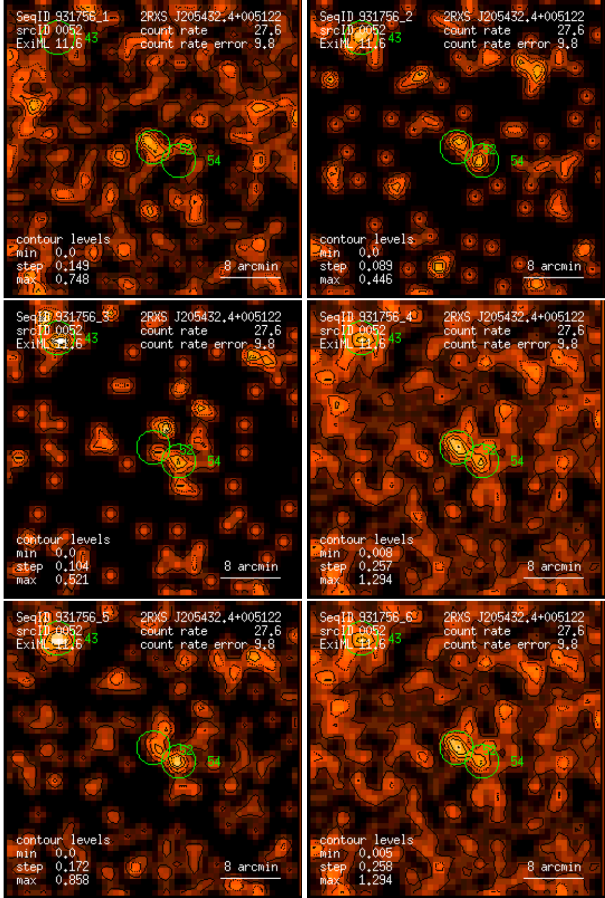
Figure 52: RASS 931756: detection 0052: band rate images, Gaussian filter: (1) PSPC channels 11 – 41, (2) 52 – 90, (3) 91 – 201, (4) 11 – 235, (5) 52 – 201, (6) 11 – 201. Broad band rates in counts/ks. Band rate contour levels in counts/ks/arcmin 2 .
