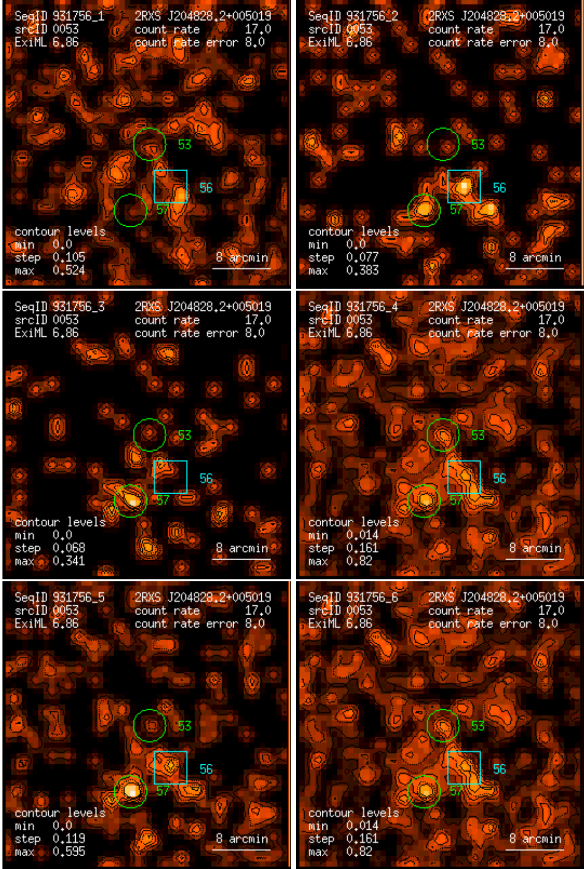
Figure 53: RASS 931756: detection 0053: band rate images, Gaussian filter: (1) PSPC channels 11 – 41, (2) 52 – 90, (3) 91 – 201, (4) 11 – 235, (5) 52 – 201, (6) 11 – 201. Broad band rates in counts/ks. Band rate contour levels in counts/ks/arcmin 2 .
