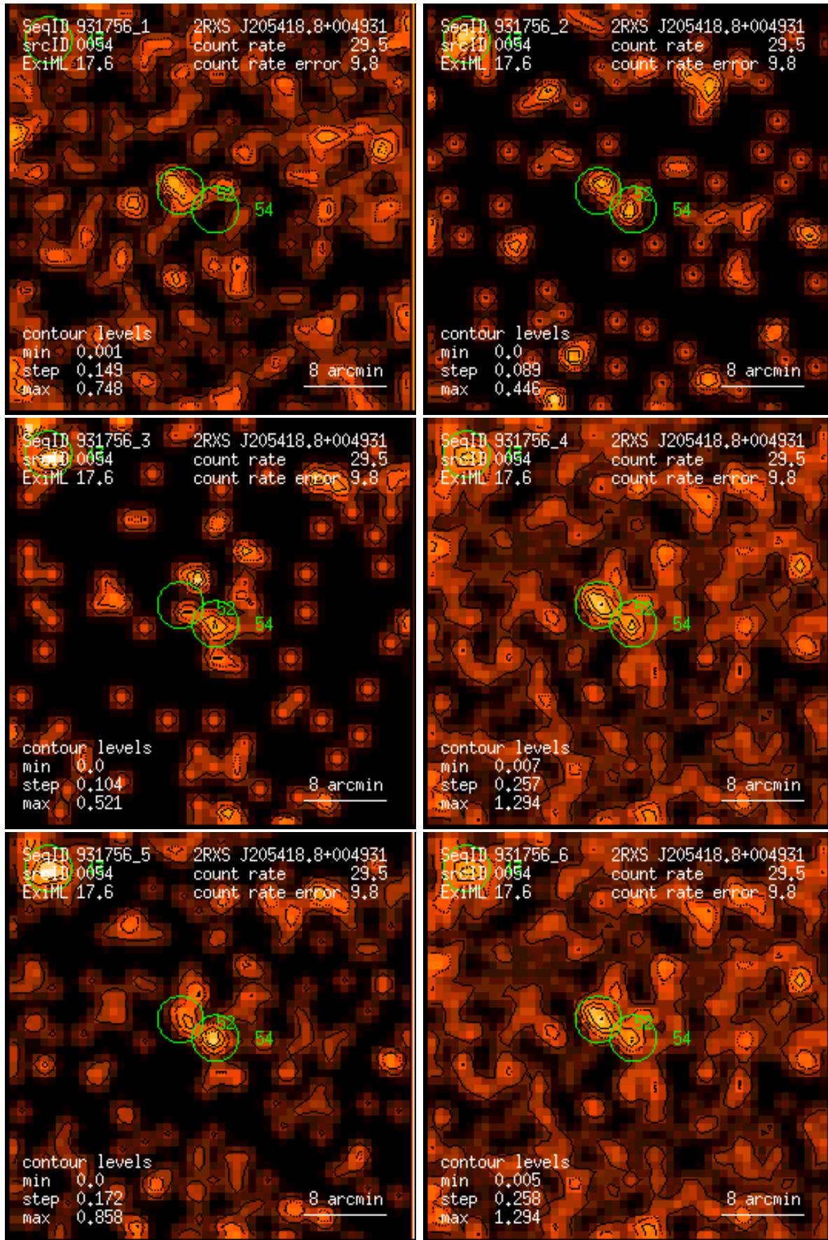
Figure 54: RASS 931756: detection 0054: band rate images, Gaussian filter: (1) PSPC channels 11 – 41, (2) 52 – 90, (3) 91 – 201, (4) 11 – 235, (5) 52 – 201, (6) 11 – 201. Broad band rates in counts/ks. Band rate contour levels in counts/ks/arcmin 2 .
