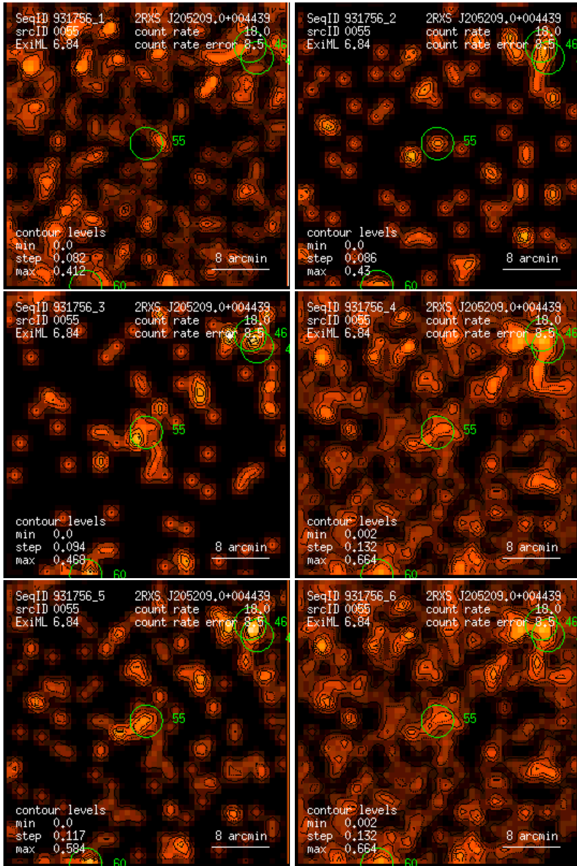
Figure 55: RASS 931756: detection 0055: band rate images, Gaussian filter: (1) PSPC channels 11 – 41, (2) 52 – 90, (3) 91 – 201, (4) 11 – 235, (5) 52 – 201, (6) 11 – 201. Broad band rates in counts/ks. Band rate contour levels in counts/ks/arcmin 2 .
