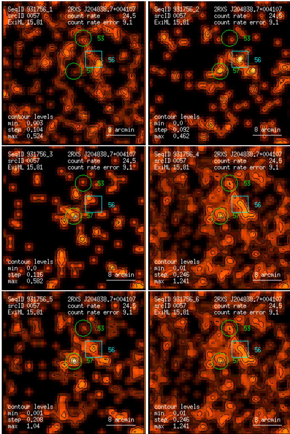
Figure 57: RASS 931756: detection 0057: band rate images, Gaussian filter: (1) PSPC channels 11 – 41, (2) 52 – 90, (3) 91 – 201, (4) 11 – 235, (5) 52 – 201, (6) 11 – 201. Broad band rates in counts/ks. Band rate contour levels in counts/ks/arcmin 2 .
