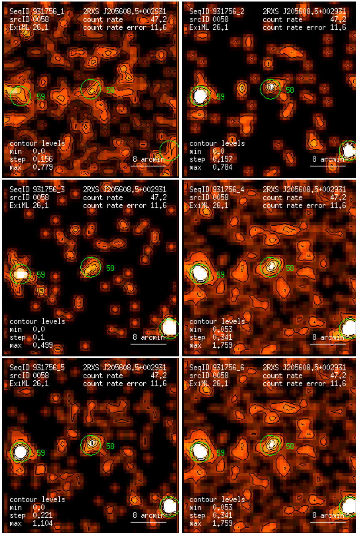
Figure 58: RASS 931756: detection 0058: band rate images, Gaussian filter: (1) PSPC channels 11 – 41, (2) 52 – 90, (3) 91 – 201, (4) 11 – 235, (5) 52 – 201, (6) 11 – 201. Broad band rates in counts/ks. Band rate contour levels in counts/ks/arcmin 2 .
