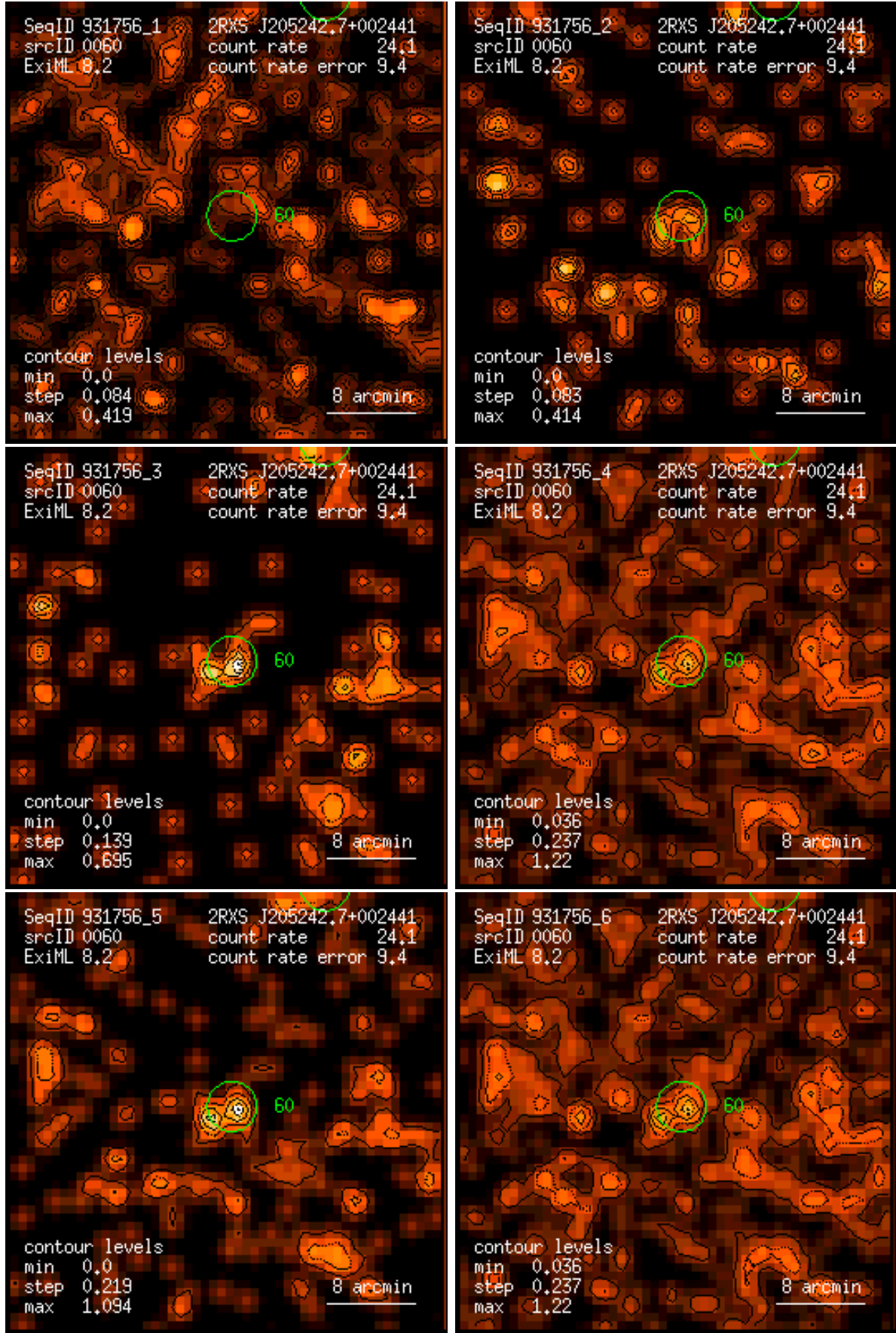
Figure 60: RASS 931756: detection 0060: band rate images, Gaussian filter: (1) PSPC channels 11 – 41, (2) 52 – 90, (3) 91 – 201, (4) 11 – 235, (5) 52 – 201, (6) 11 – 201. Broad band rates in counts/ks. Band rate contour levels in counts/ks/arcmin 2 .
