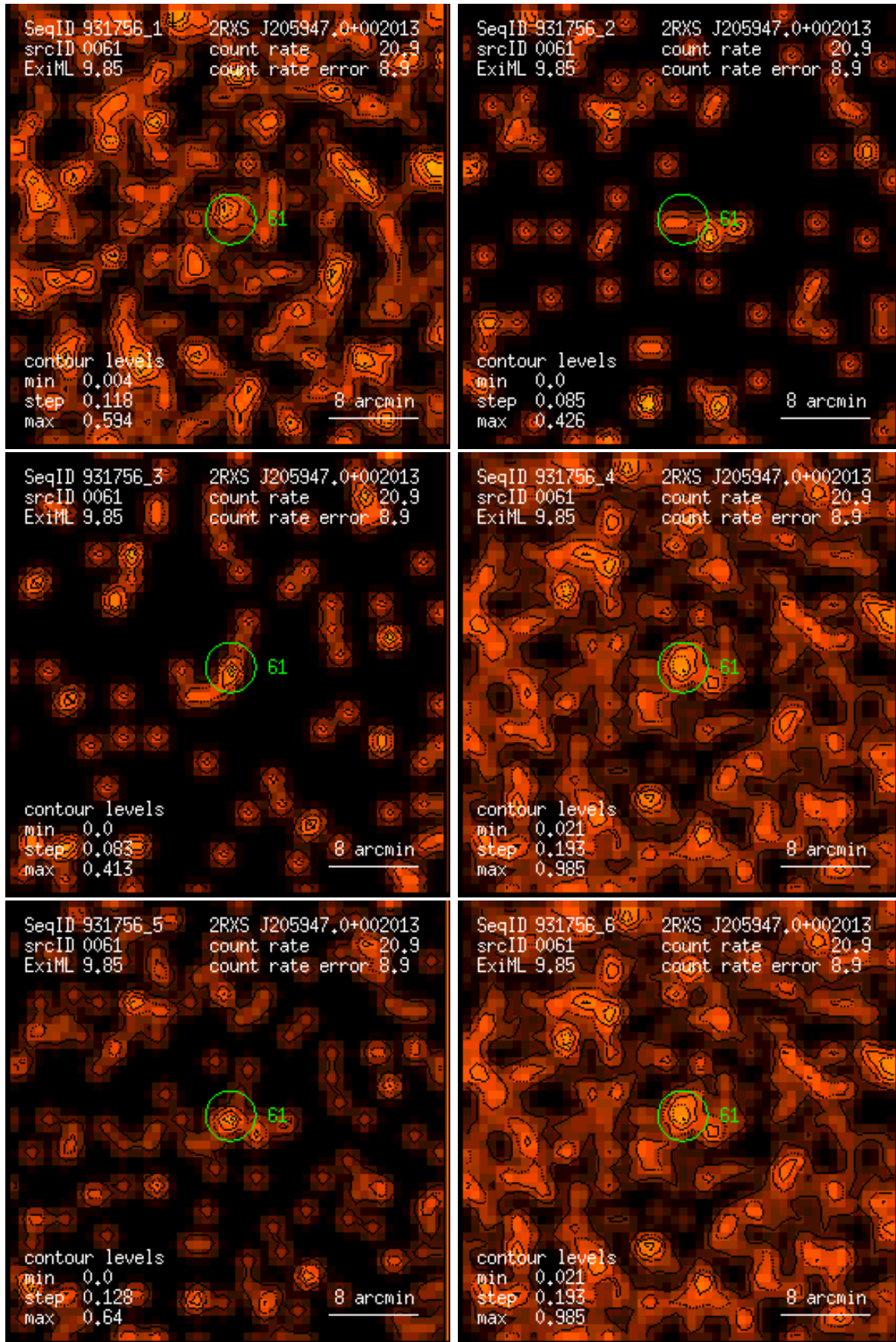
Figure 61: RASS 931756: detection 0061: band rate images, Gaussian filter: (1) PSPC channels 11 – 41, (2) 52 – 90, (3) 91 – 201, (4) 11 – 235, (5) 52 – 201, (6) 11 – 201. Broad band rates in counts/ks. Band rate contour levels in counts/ks/arcmin 2 .
