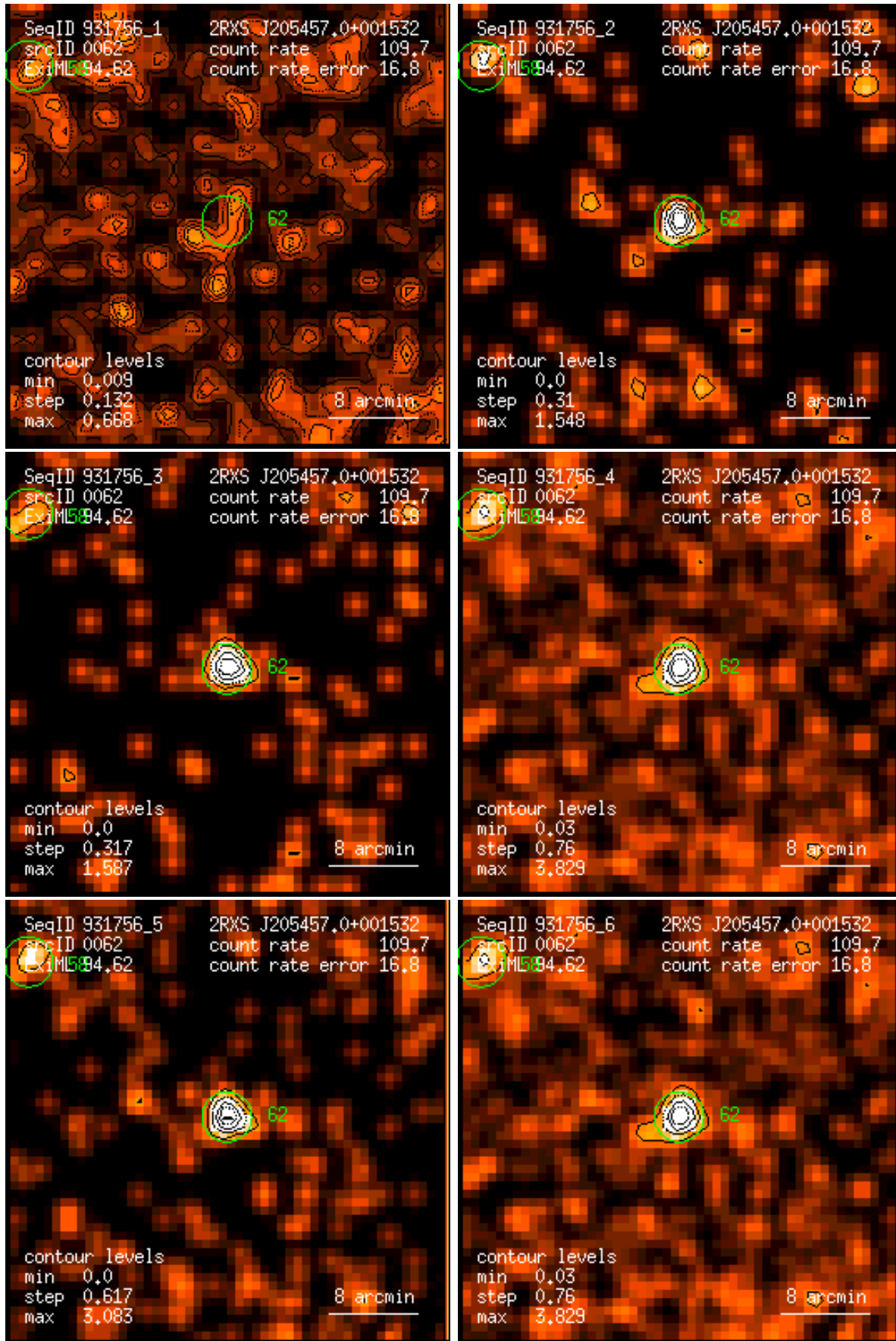
Figure 62: RASS 931756: detection 0062: band rate images, Gaussian filter: (1) PSPC channels 11 – 41, (2) 52 – 90, (3) 91 – 201, (4) 11 – 235, (5) 52 – 201, (6) 11 – 201. Broad band rates in counts/ks. Band rate contour levels in counts/ks/arcmin 2 .
