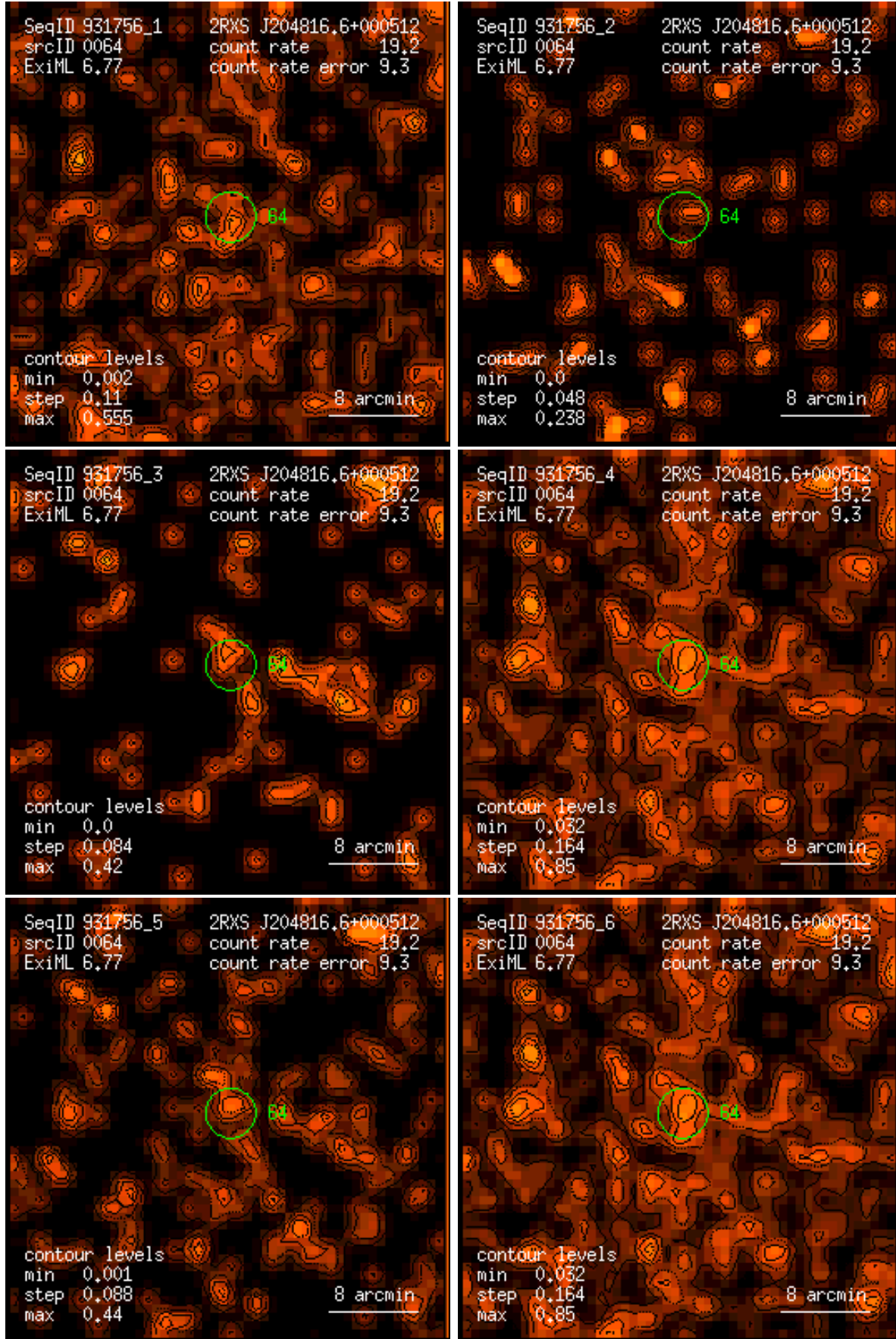
Figure 64: RASS 931756: detection 0064: band rate images, Gaussian filter: (1) PSPC channels 11 – 41, (2) 52 – 90, (3) 91 – 201, (4) 11 – 235, (5) 52 – 201, (6) 11 – 201. Broad band rates in counts/ks. Band rate contour levels in counts/ks/arcmin 2 .
