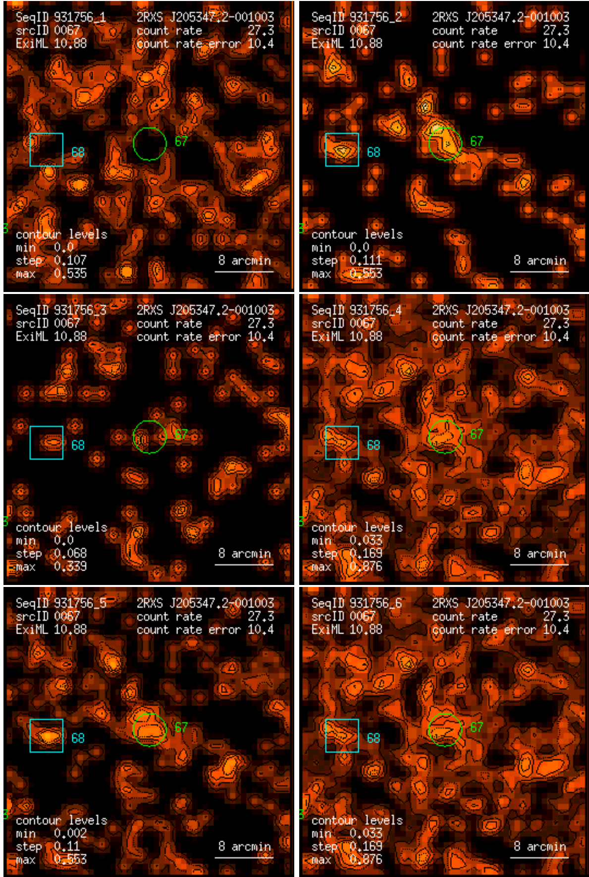
Figure 67: RASS 931756: detection 0067: band rate images, Gaussian filter: (1) PSPC channels 11 – 41, (2) 52 – 90, (3) 91 – 201, (4) 11 – 235, (5) 52 – 201, (6) 11 – 201. Broad band rates in counts/ks. Band rate contour levels in counts/ks/arcmin 2 .
