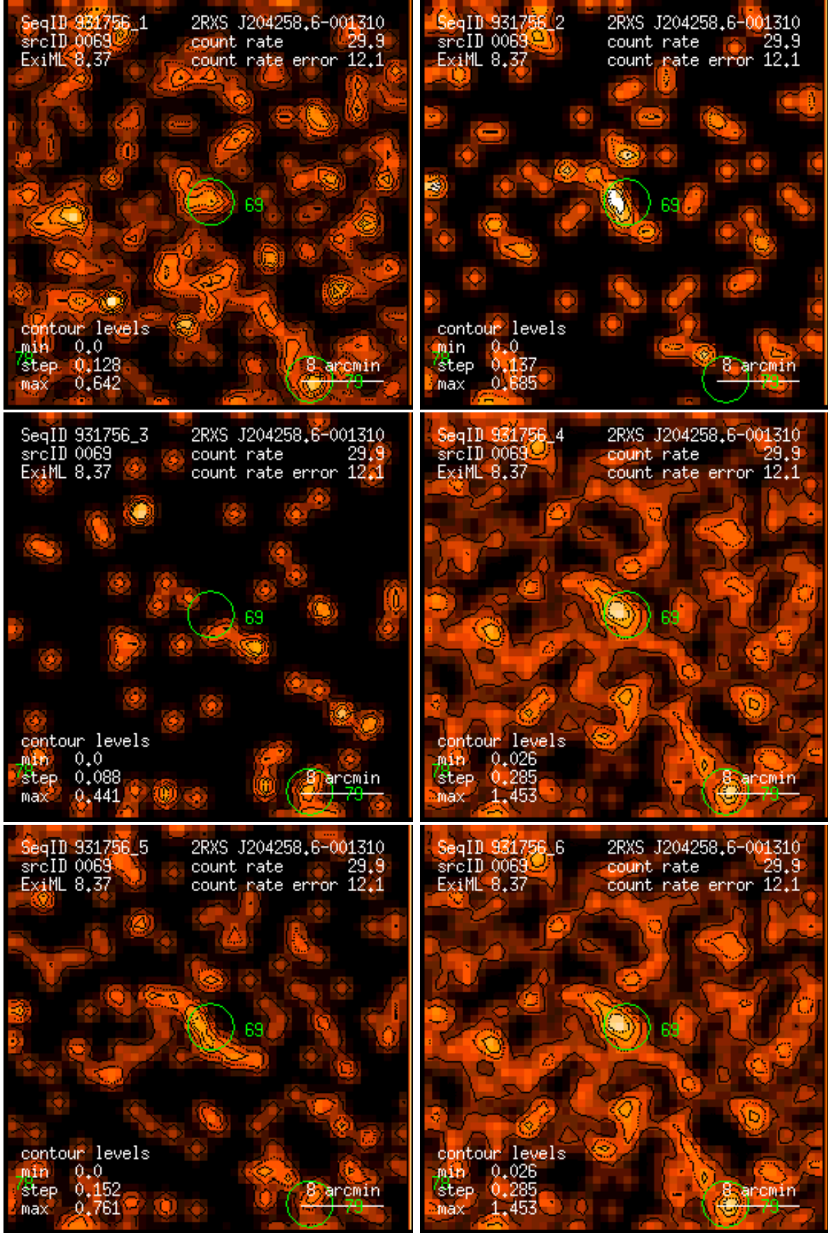
Figure 69: RASS 931756: detection 0069: band rate images, Gaussian filter: (1) PSPC channels 11 – 41, (2) 52 – 90, (3) 91 – 201, (4) 11 – 235, (5) 52 – 201, (6) 11 – 201. Broad band rates in counts/ks. Band rate contour levels in counts/ks/arcmin 2 .
