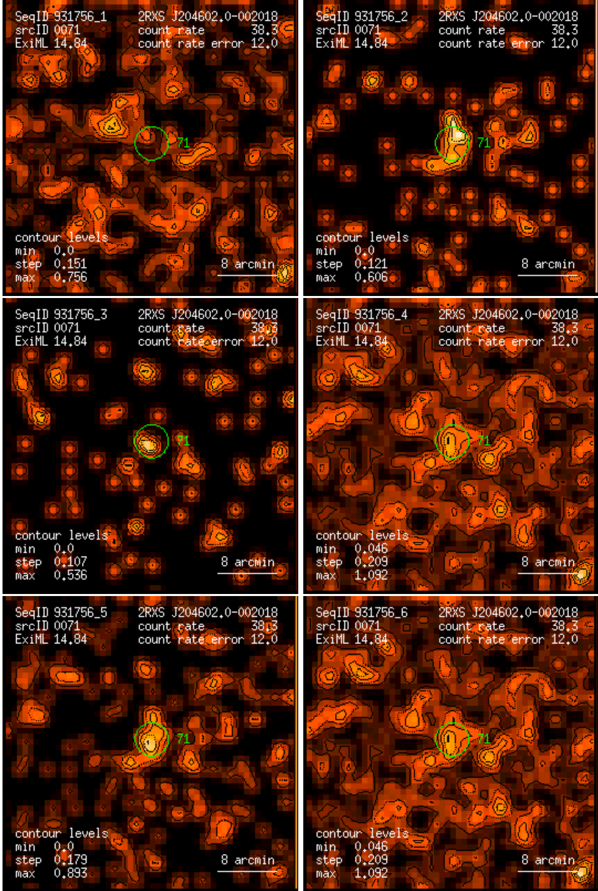
Figure 71: RASS 931756: detection 0071: band rate images, Gaussian filter: (1) PSPC channels 11 – 41, (2) 52 – 90, (3) 91 – 201, (4) 11 – 235, (5) 52 – 201, (6) 11 – 201. Broad band rates in counts/ks. Band rate contour levels in counts/ks/arcmin 2 .
