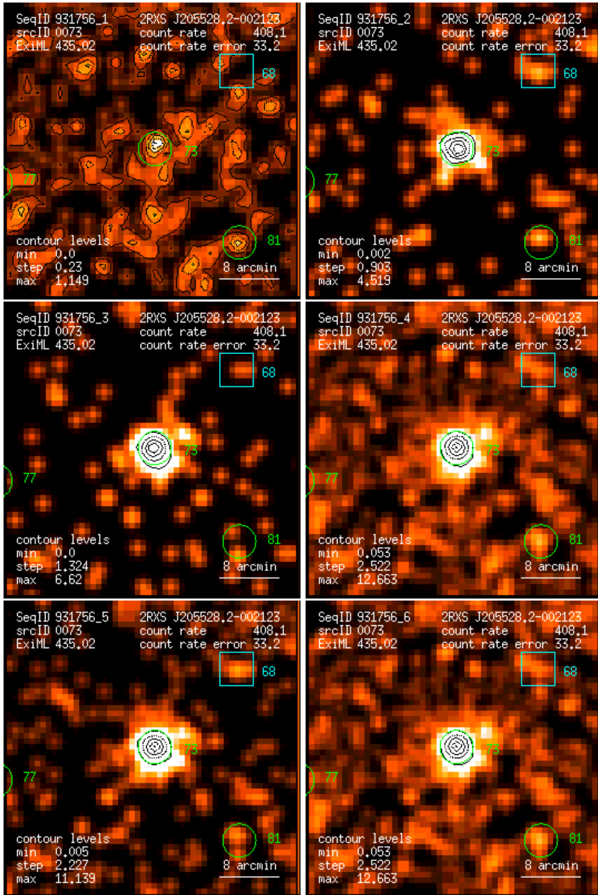
Figure 73: RASS 931756: detection 0073: band rate images, Gaussian filter: (1) PSPC channels 11 – 41, (2) 52 – 90, (3) 91 – 201, (4) 11 – 235, (5) 52 – 201, (6) 11 – 201. Broad band rates in counts/ks. Band rate contour levels in counts/ks/arcmin 2 .
