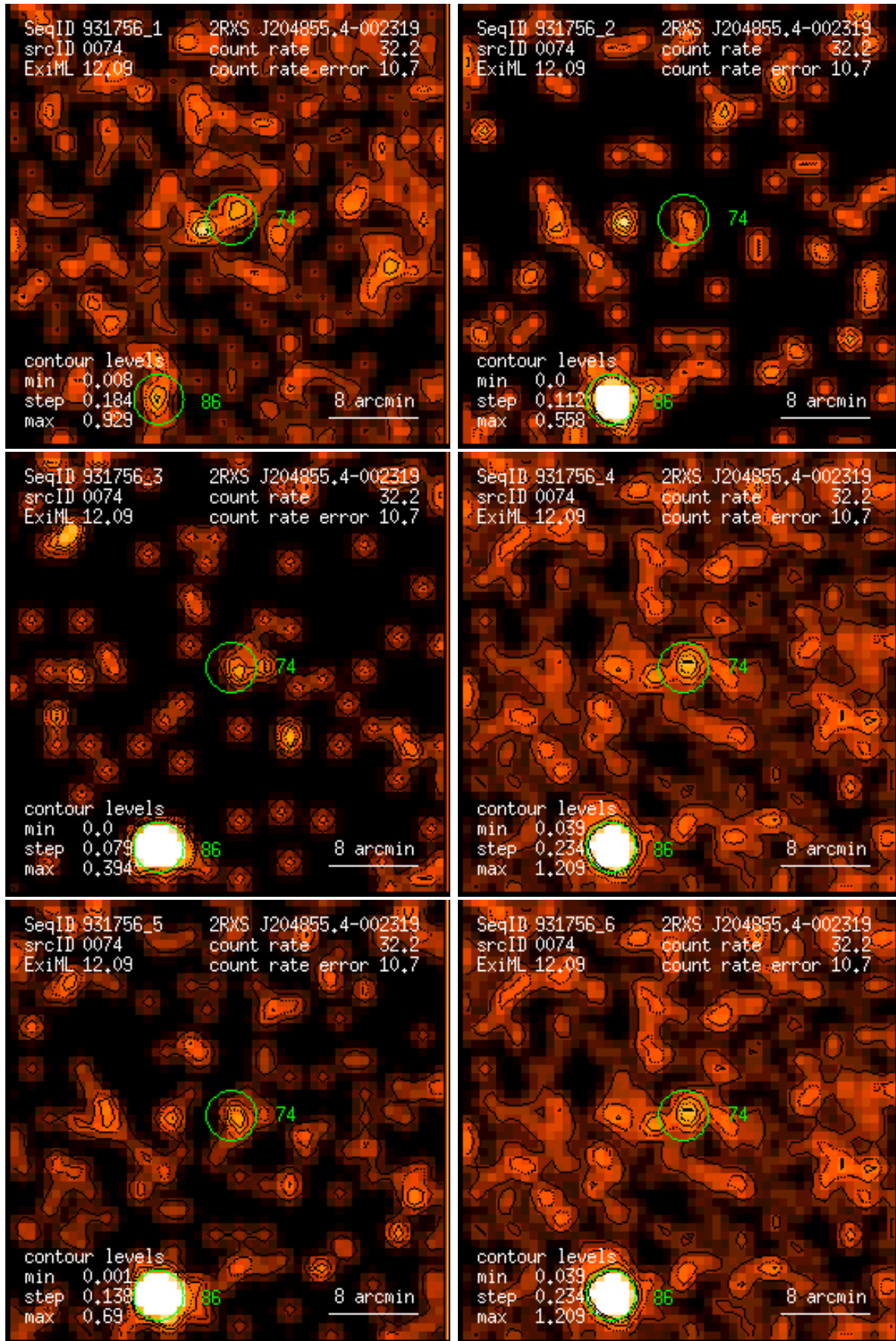
Figure 74: RASS 931756: detection 0074: band rate images, Gaussian filter: (1) PSPC channels 11 – 41, (2) 52 – 90, (3) 91 – 201, (4) 11 – 235, (5) 52 – 201, (6) 11 – 201. Broad band rates in counts/ks. Band rate contour levels in counts/ks/arcmin 2 .
