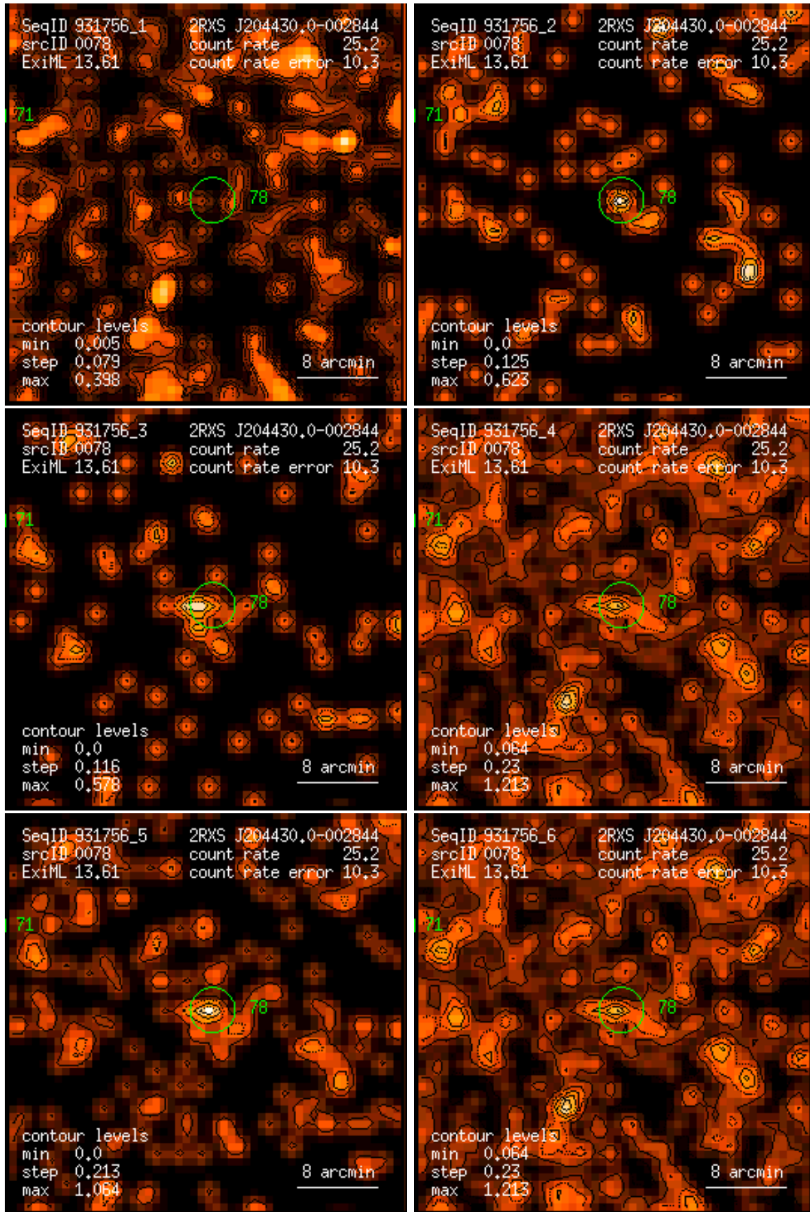
Figure 78: RASS 931756: detection 0078: band rate images, Gaussian filter: (1) PSPC channels 11 – 41, (2) 52 – 90, (3) 91 – 201, (4) 11 – 235, (5) 52 – 201, (6) 11 – 201. Broad band rates in counts/ks. Band rate contour levels in counts/ks/arcmin 2 .
