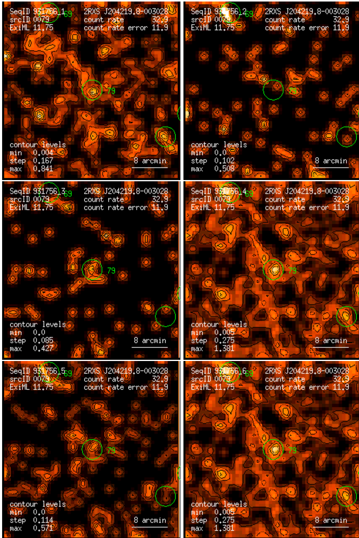
Figure 79: RASS 931756: detection 0079: band rate images, Gaussian filter: (1) PSPC channels 11 – 41, (2) 52 – 90, (3) 91 – 201, (4) 11 – 235, (5) 52 – 201, (6) 11 – 201. Broad band rates in counts/ks. Band rate contour levels in counts/ks/arcmin 2 .
