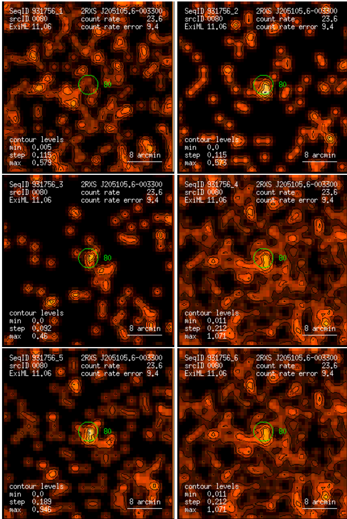
Figure 80: RASS 931756: detection 0080: band rate images, Gaussian filter: (1) PSPC channels 11 – 41, (2) 52 – 90, (3) 91 – 201, (4) 11 – 235, (5) 52 – 201, (6) 11 – 201. Broad band rates in counts/ks. Band rate contour levels in counts/ks/arcmin 2 .
