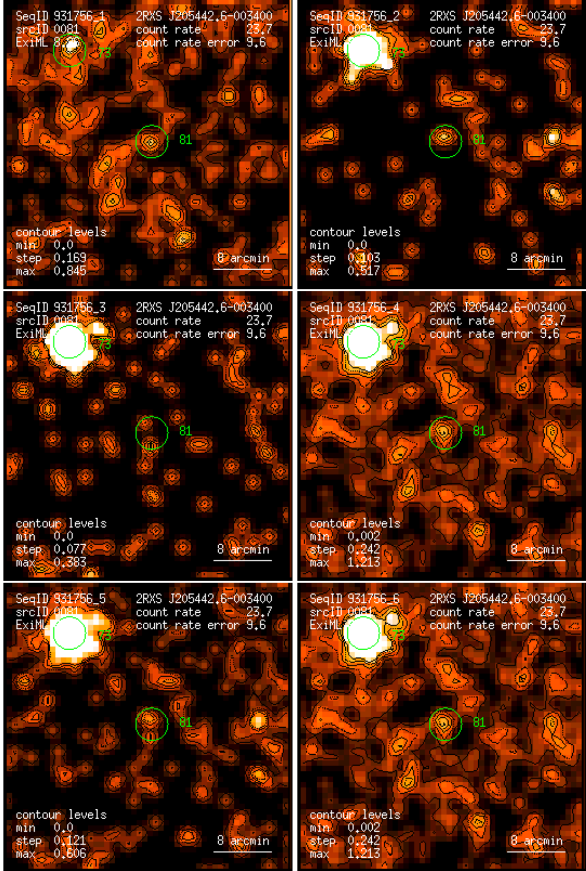
Figure 81: RASS 931756: detection 0081: band rate images, Gaussian filter: (1) PSPC channels 11 – 41, (2) 52 – 90, (3) 91 – 201, (4) 11 – 235, (5) 52 – 201, (6) 11 – 201. Broad band rates in counts/ks. Band rate contour levels in counts/ks/arcmin 2 .
